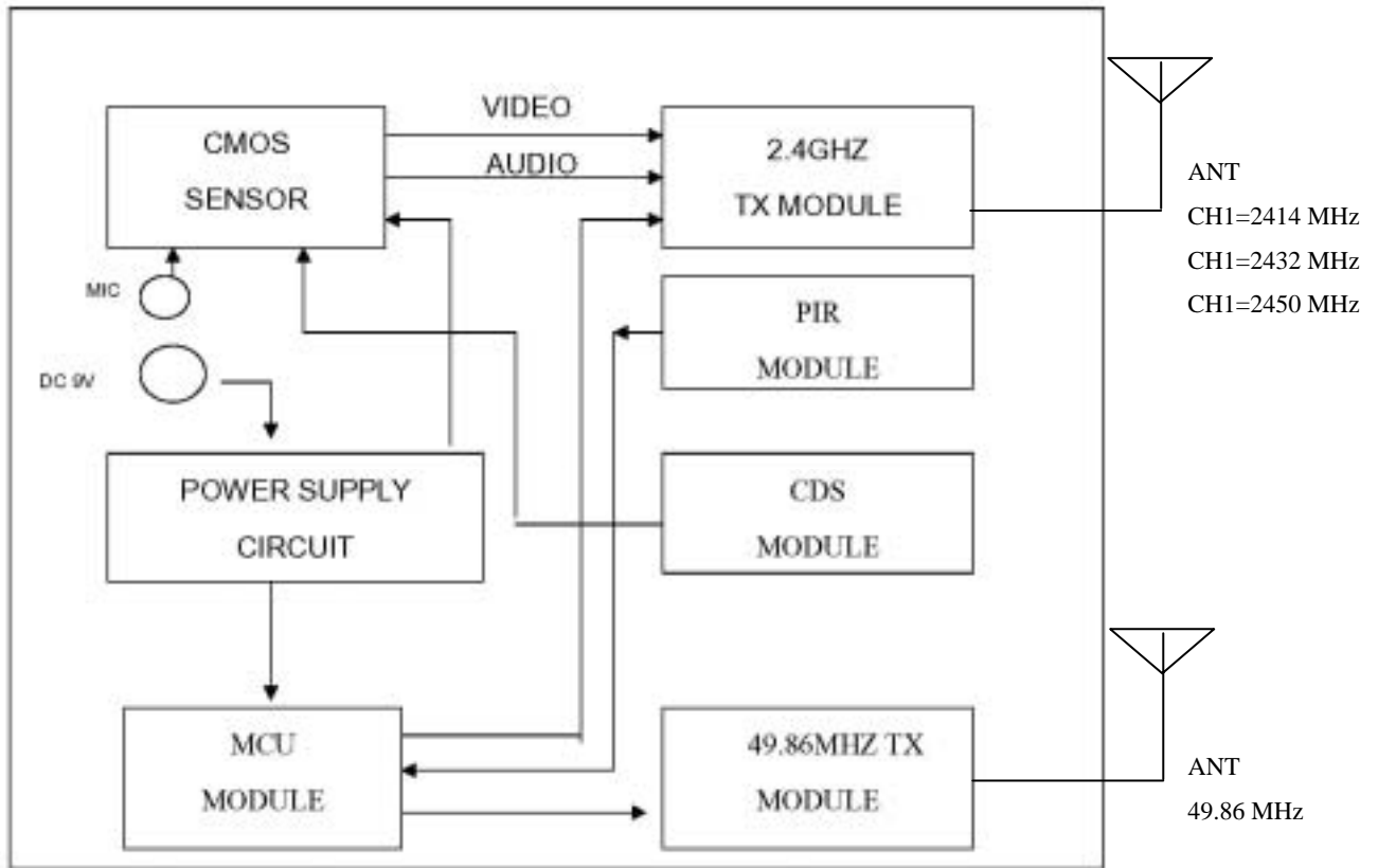
SB-102BWC BLOCK DIAGRAM
