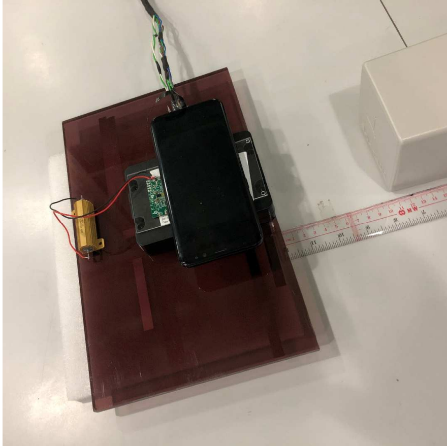
Test Setup Photo: Worst case
