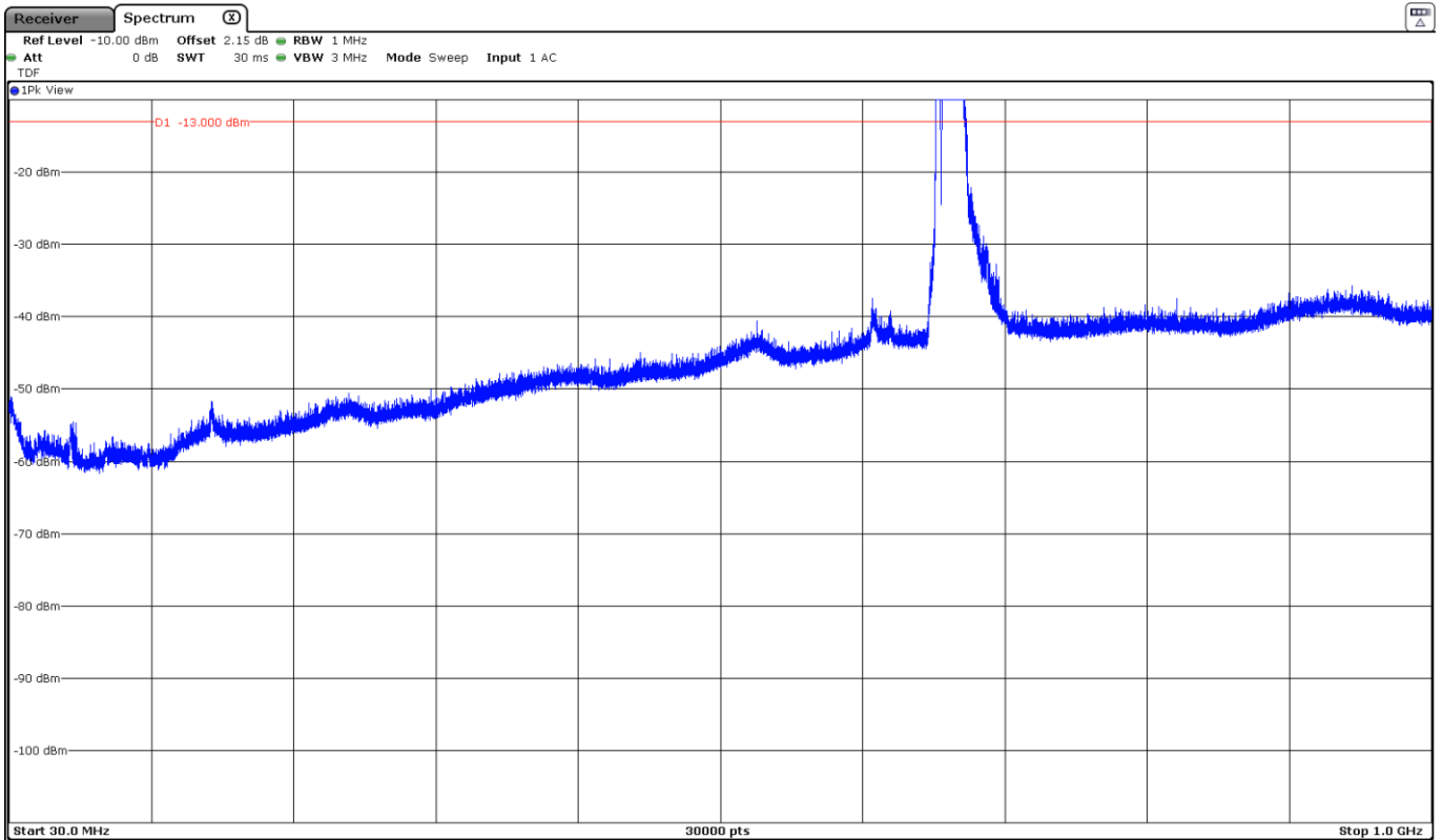
The peaks at 670.5MHz (n71A) and 688MHz (LTE 71) to above the limit are the carrier frequencies.
