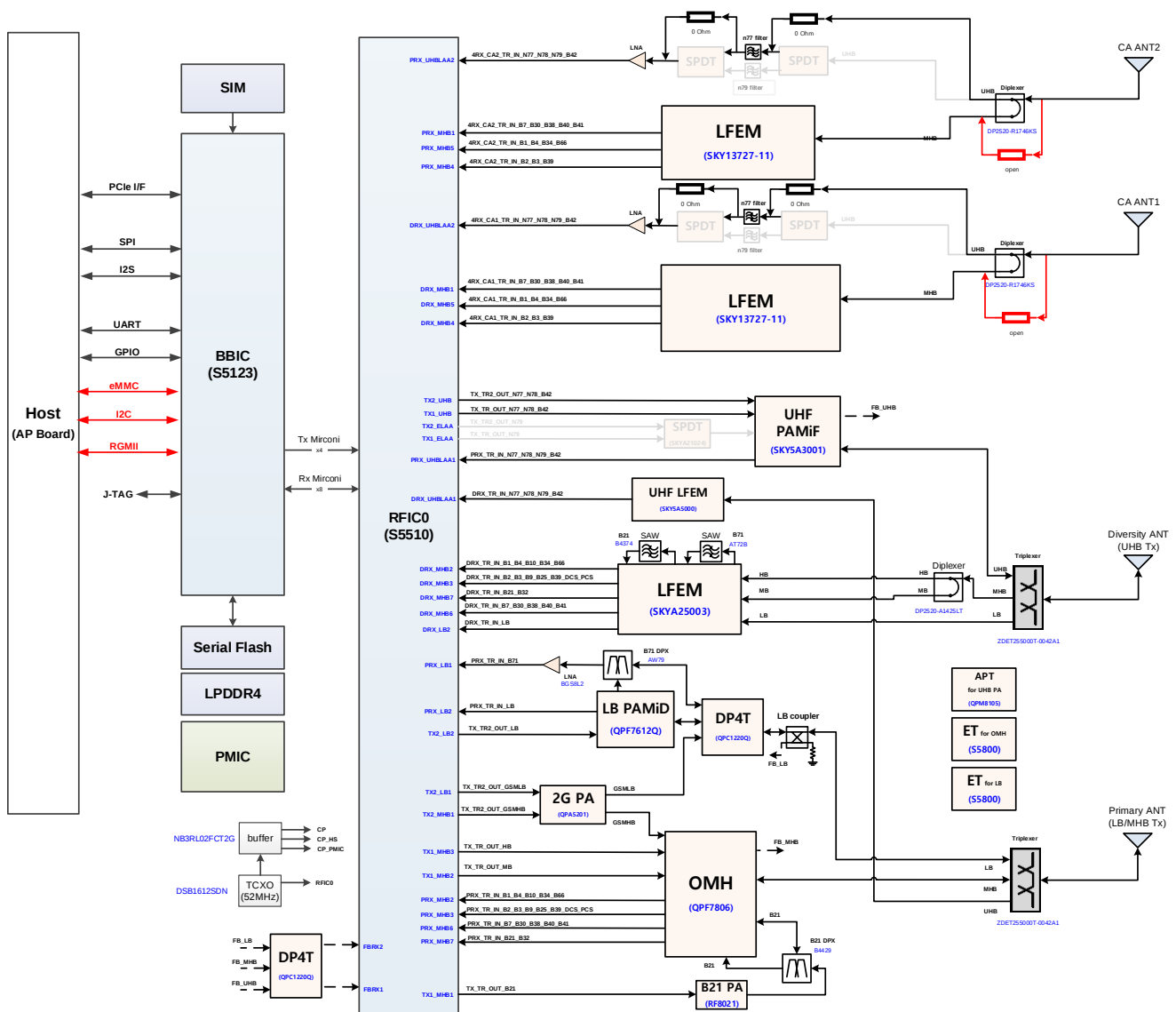
Figure 1-1 Circuit block diagram of the module
