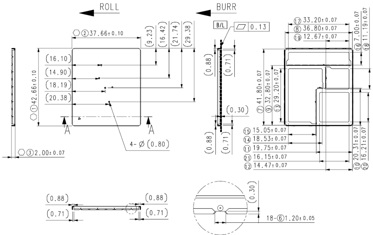
Figure 6-2 Shield-can cover
