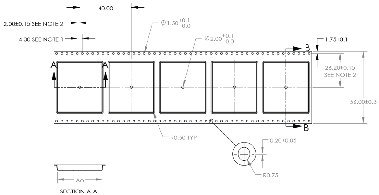
Figure 6-3 Packaging
