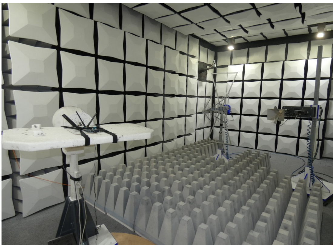
Photo 2: Test setup for radiated measurements above 1 GHz
