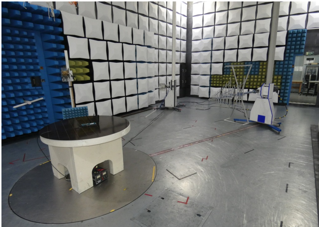
Photo 1: Test setup for radiated measurements below 1 GHz
