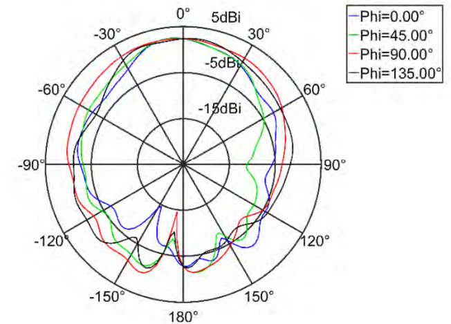
radiation pattern of the antenna realized gain (E_Total, Freq = 2500.00 MHz)
