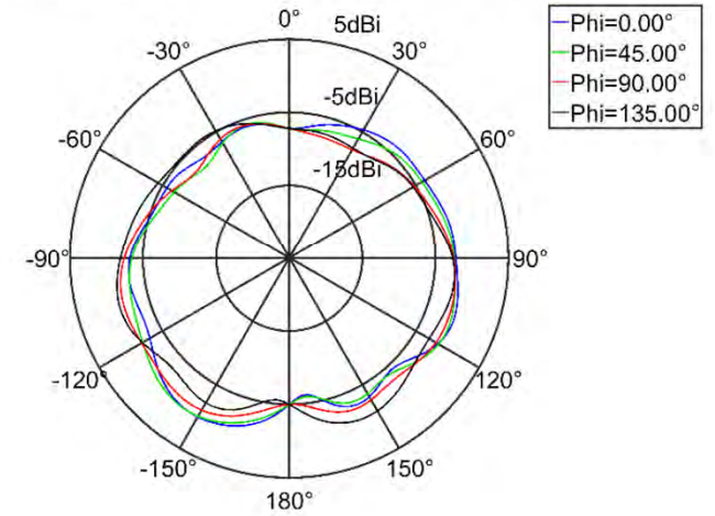
radiation pattern of the antenna realized gain (E_Total, Freq = 1462.90 MHz)
