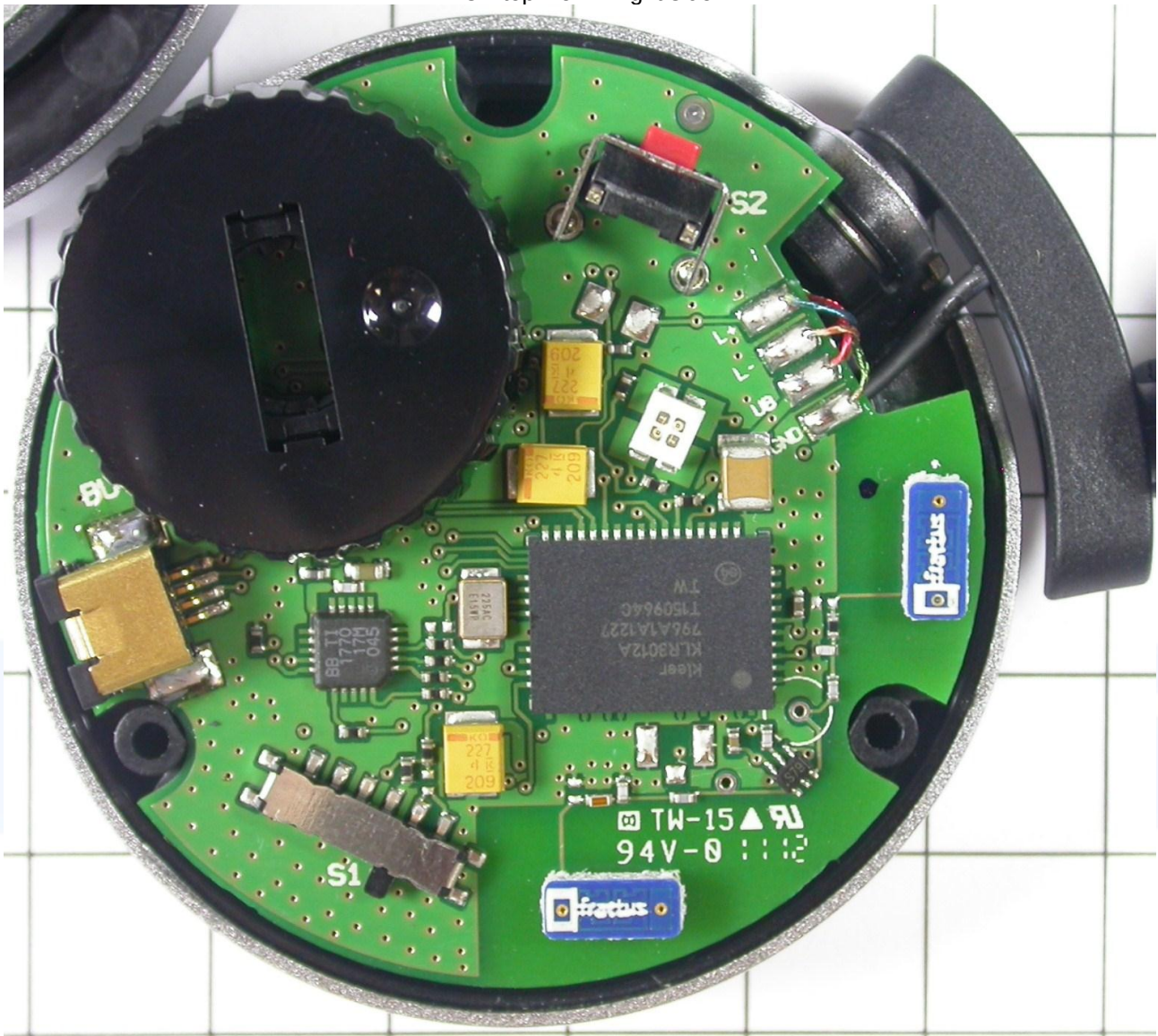
PCB top view – right side
