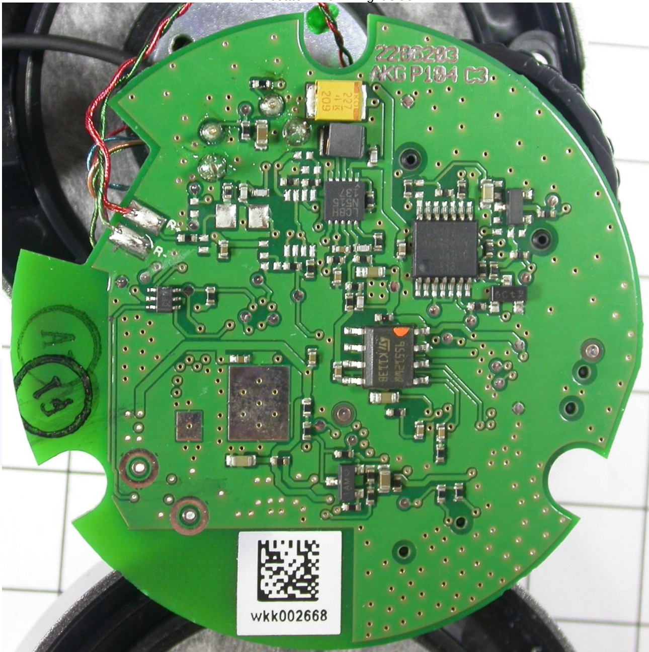
PCB bottom view – right side
