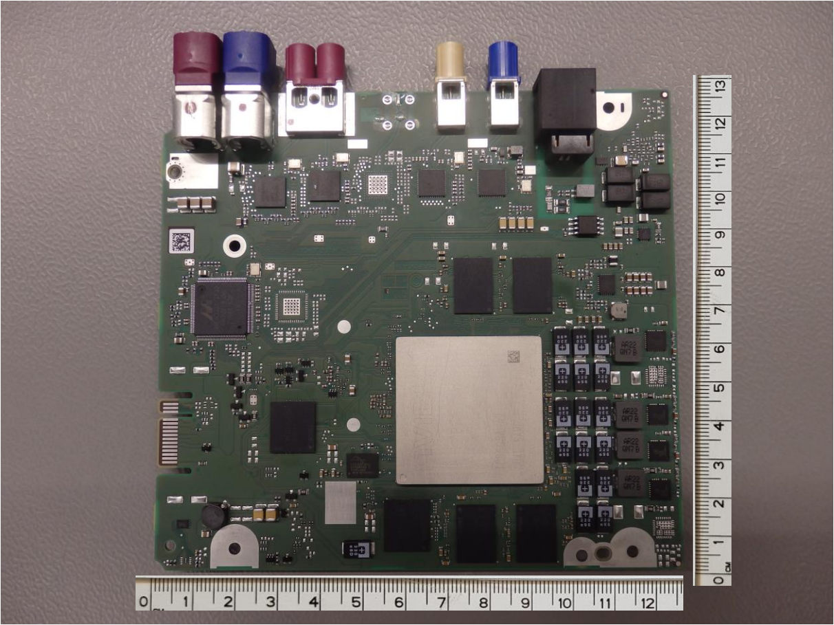
PCBA_MMB_3860388 top / bottom (125 x 125 mm)
