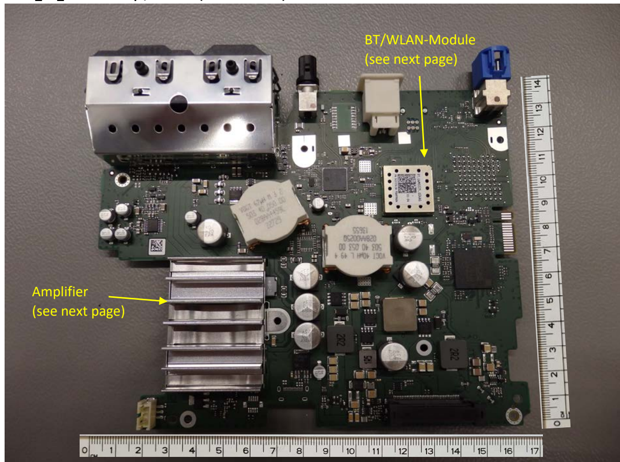
PCBA_BB_3899616 top / bottom (168 x 136 mm)
