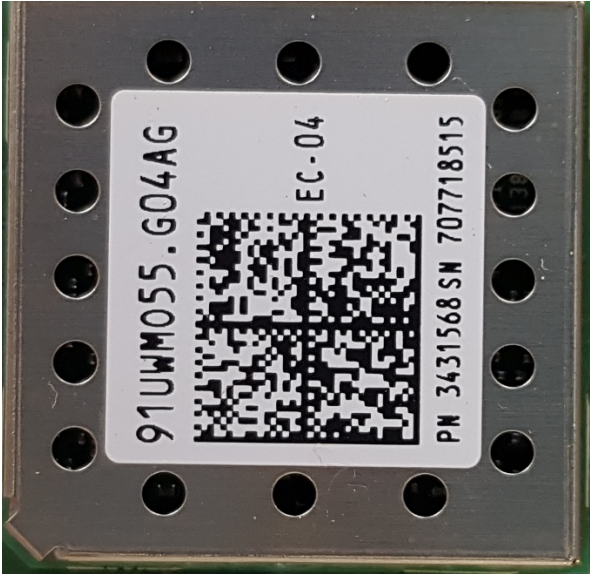
BT/WLAN-Module with shielding plate (20x20mm)
