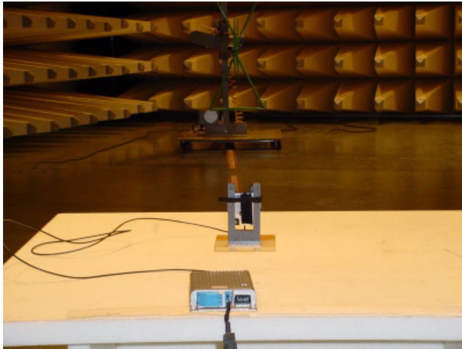
Photo 1: Radiated Emissions
