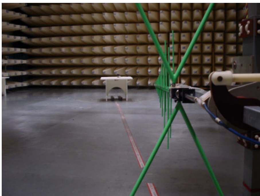
Photo 2: Radiated Emissions
