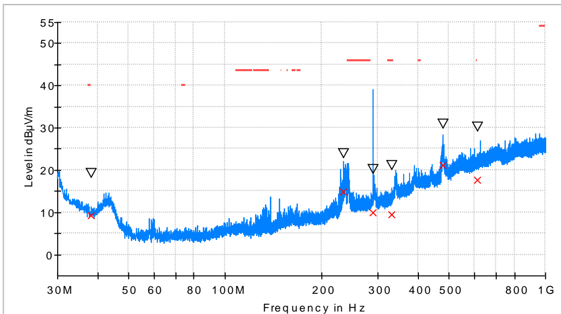
RF_FCC_15.247_E Field_30MHz_1GHz
