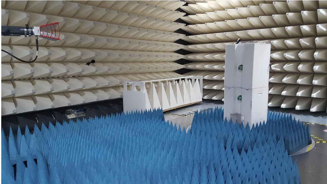
Figure D7. Radiated emission Setup 2
