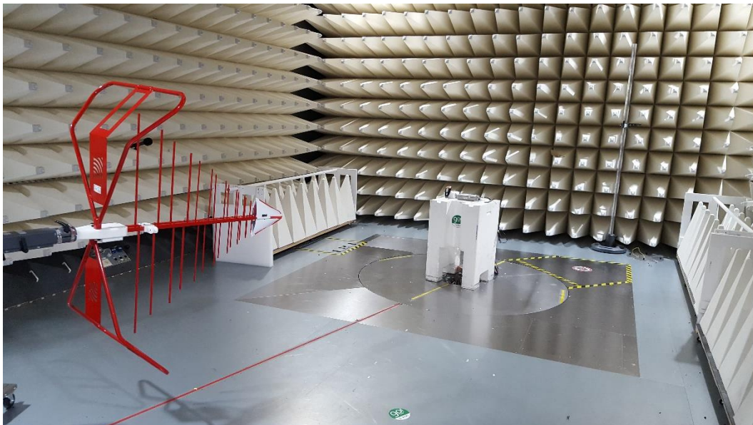
Figure D6. Radiated emission Setup 2
