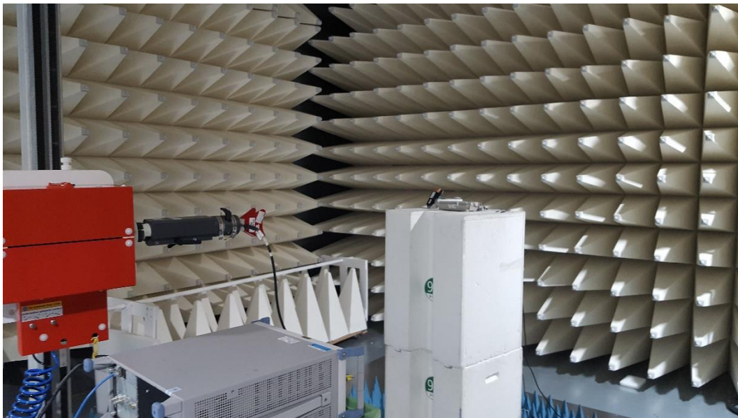
Figure D8. Radiated emission Setup 3
