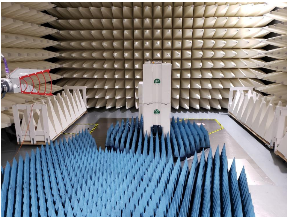
Figure C6. High Range Radiated Emission test setup 1
