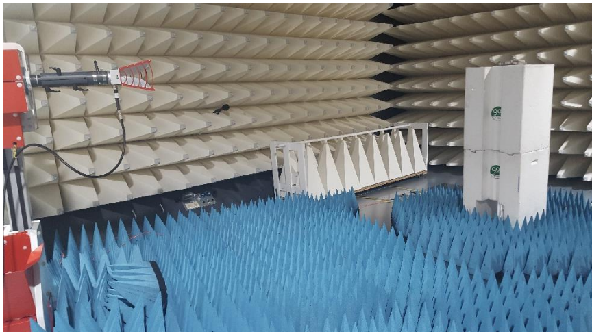
Figure C6. High Range Radiated Emission test setup 1-18GHz
