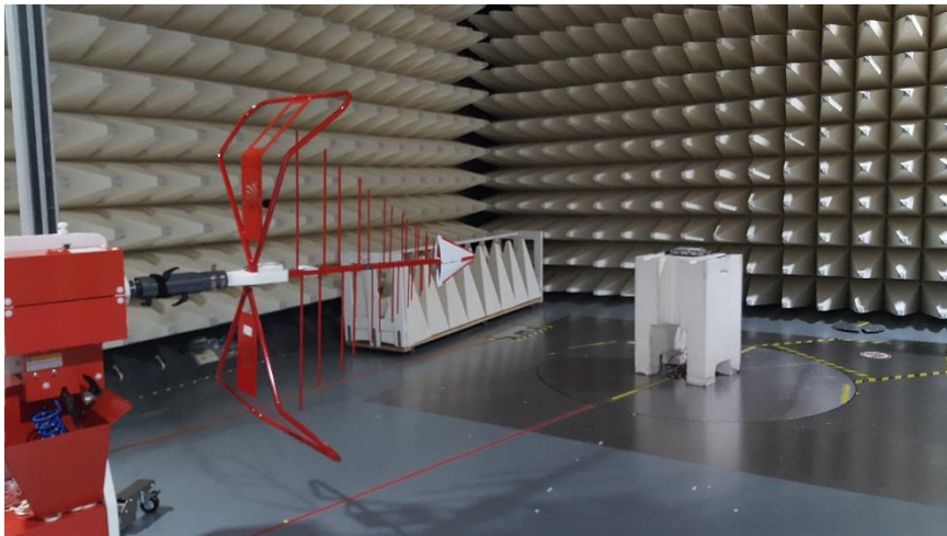
Figure C5. Low Range Radiated Emission test setup
