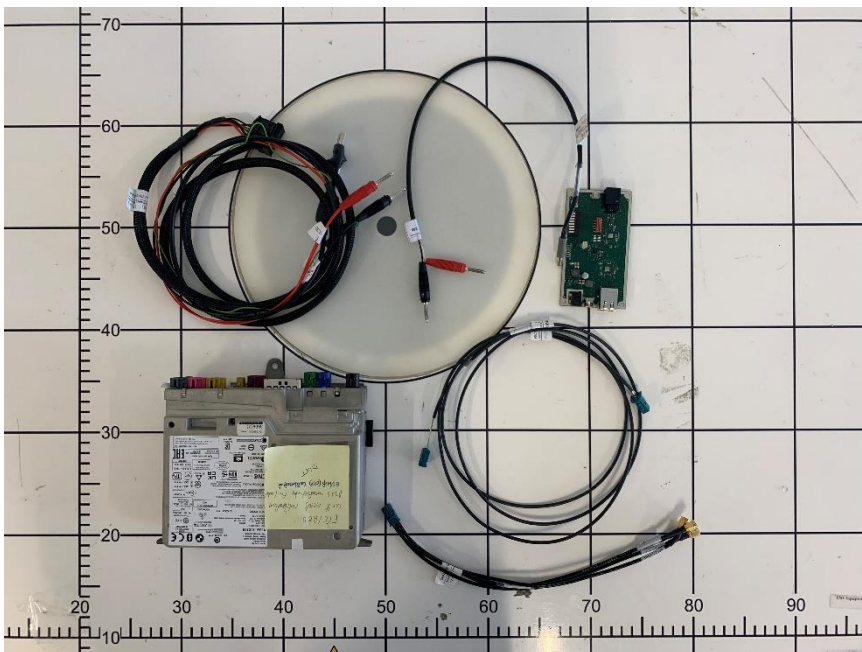
Figure C4. Front View of DUT with Accessories
