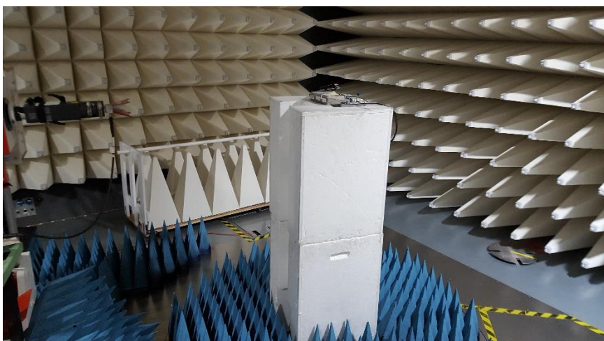
Figure C7. High Range Radiated Emission test setup 18-40GHz
