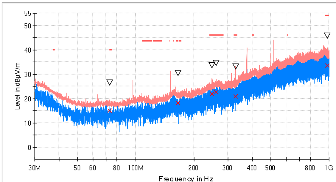
RF_FCC_15.407_E Field_30MHz_1GHz
