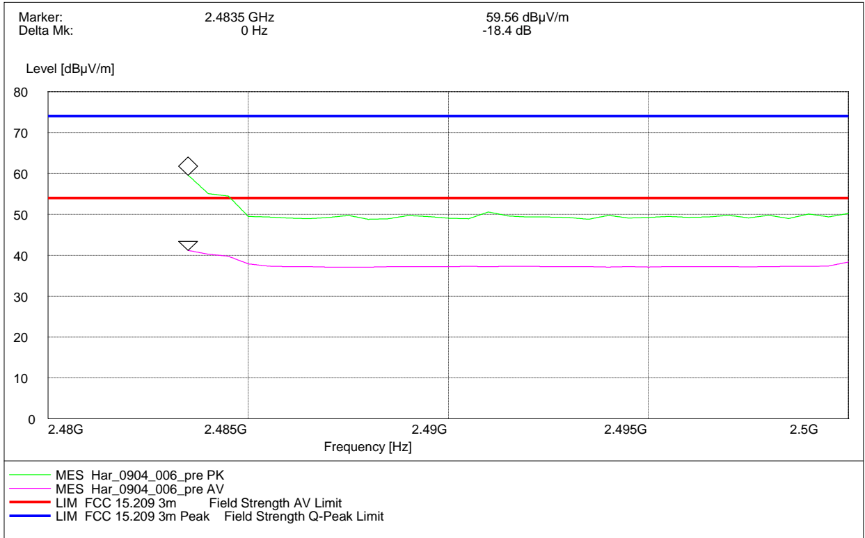
Radiated measurement (higher band edge)
