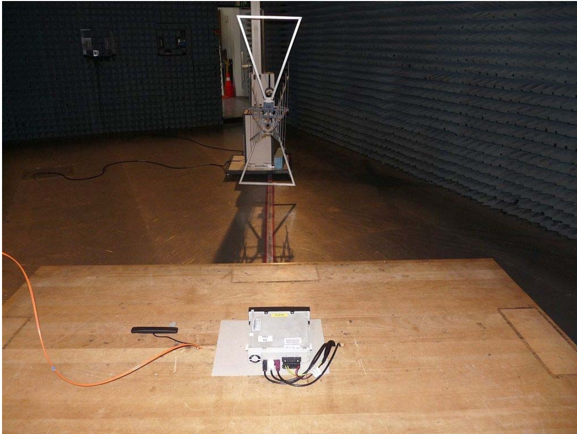
Photo 2: Test setup for radiated measurements (Enclosure, semi-anechoic chamber, 30 MHz to 1 GHz, intentional radiator §15, EUT NBT RSE / 43090a01)
