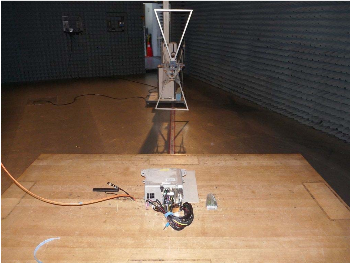
Photo 2: Test setup for radiated measurements (Enclosure, semi-anechoic chamber, 30 MHz to 1 GHz, intentional radiator §15, EUT NBT HU / 43080a01)
