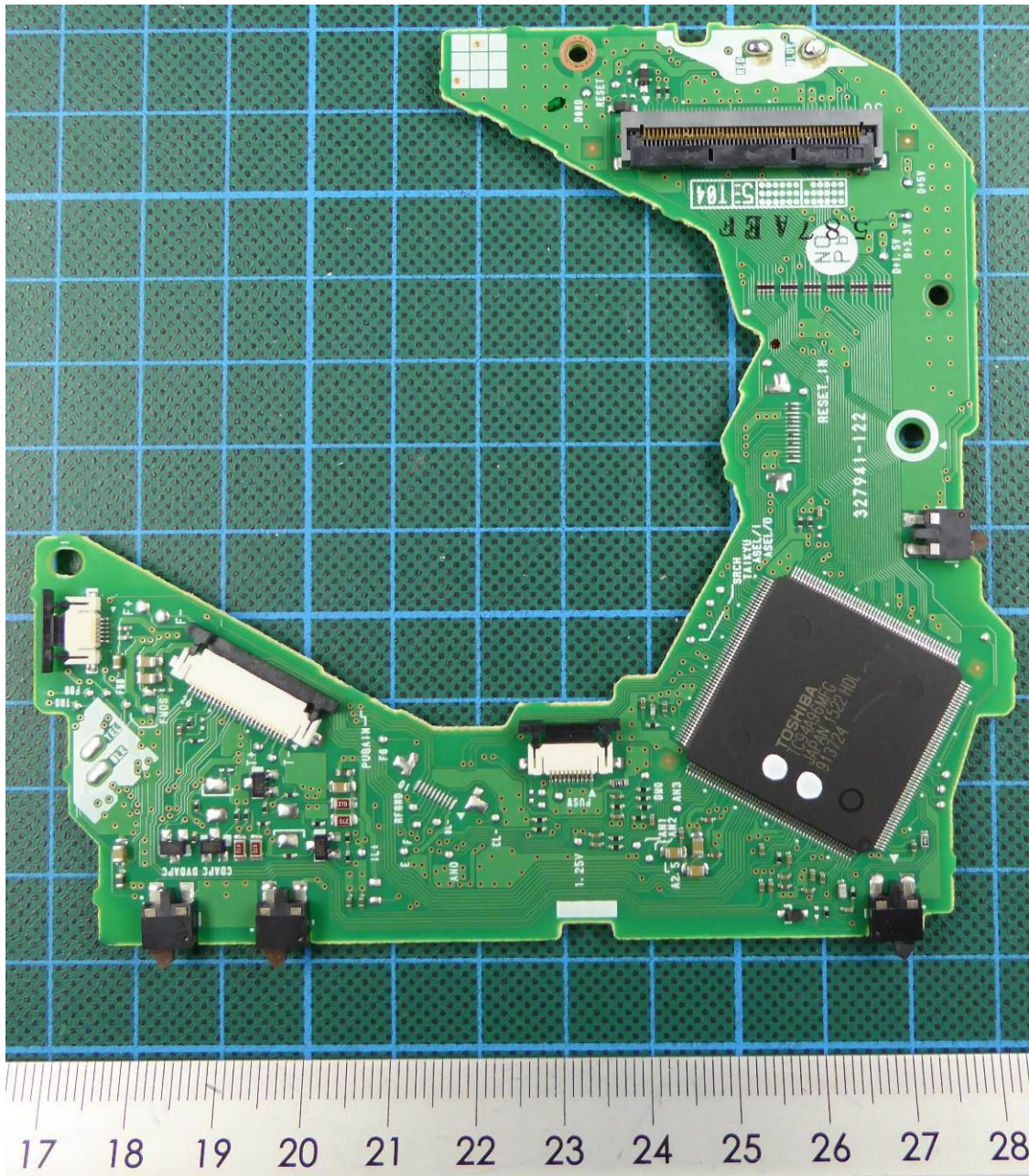
160090_26. jpg: EUT – Main Unit – CD drive PCB top view
