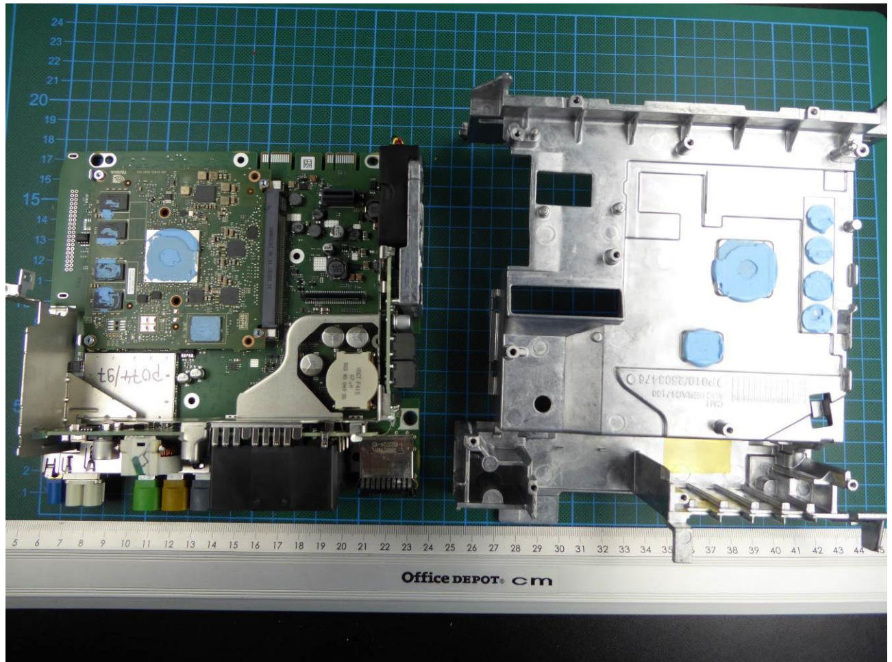
160090_35. jpg: EUT – Main Unit – with Main PCB
