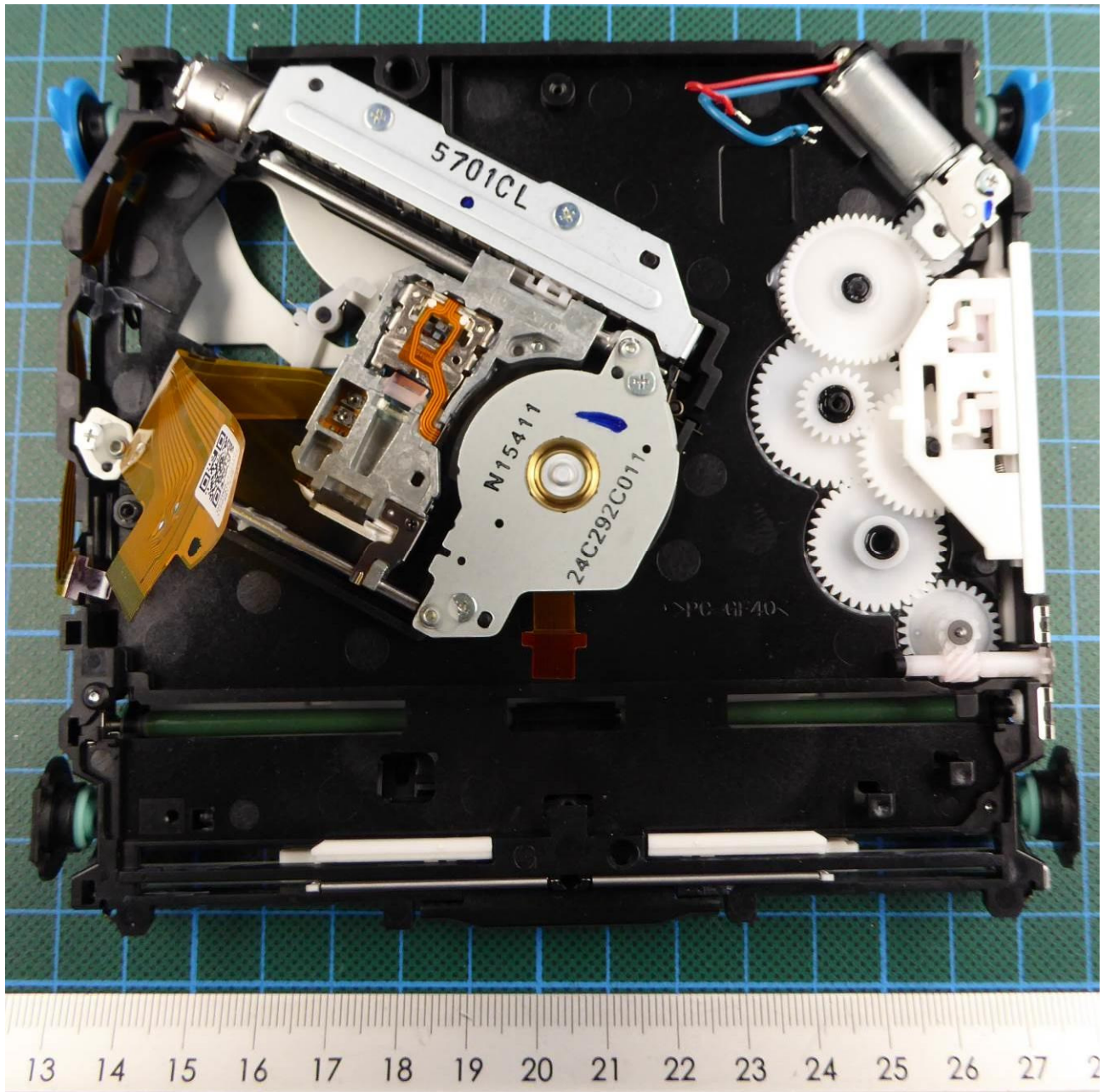
160090_29. jpg: EUT – Main Unit – CD drive without PCB bottom view
