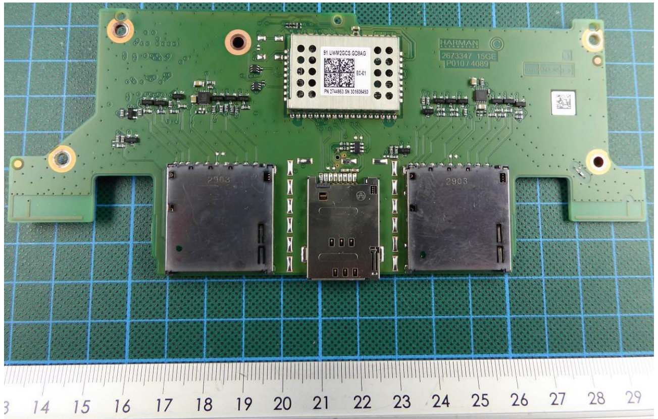
160090_32. jpg: EUT – Main Unit – RF PCB top view
