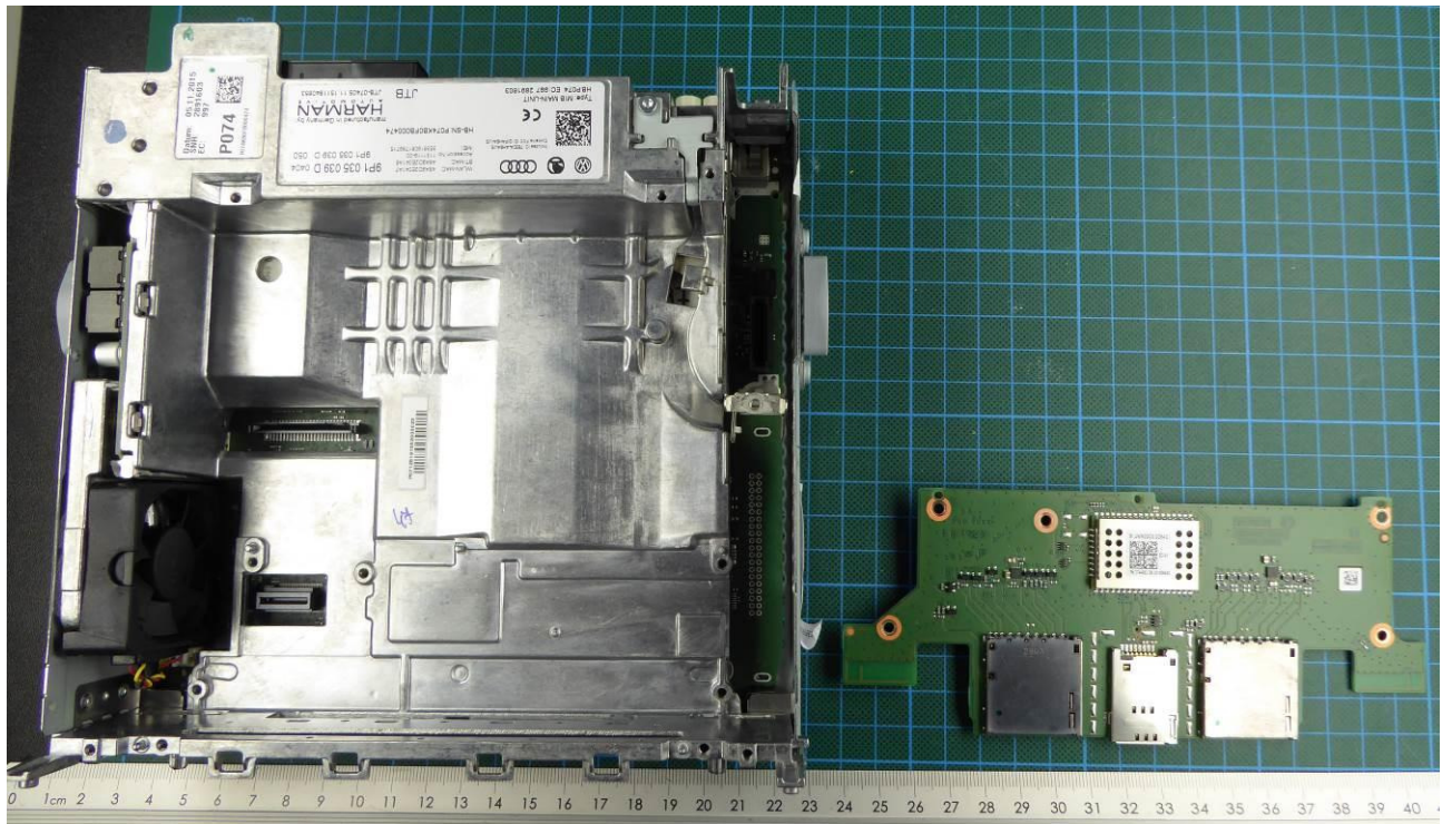
160090_30. jpg: EUT – Main Unit without RF PCB
