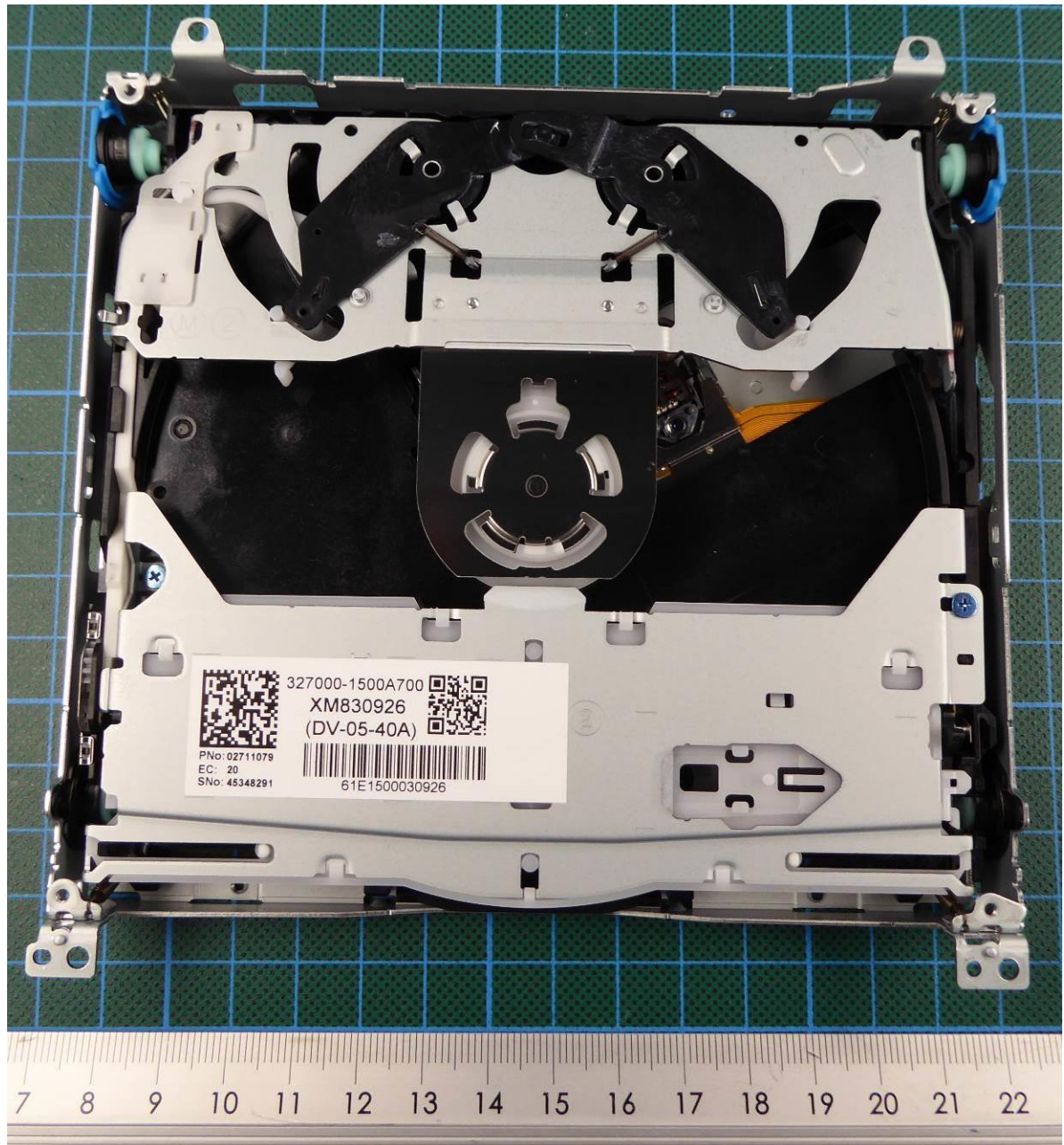
160090_28. jpg: EUT – Main Unit – CD drive without PCB top view
