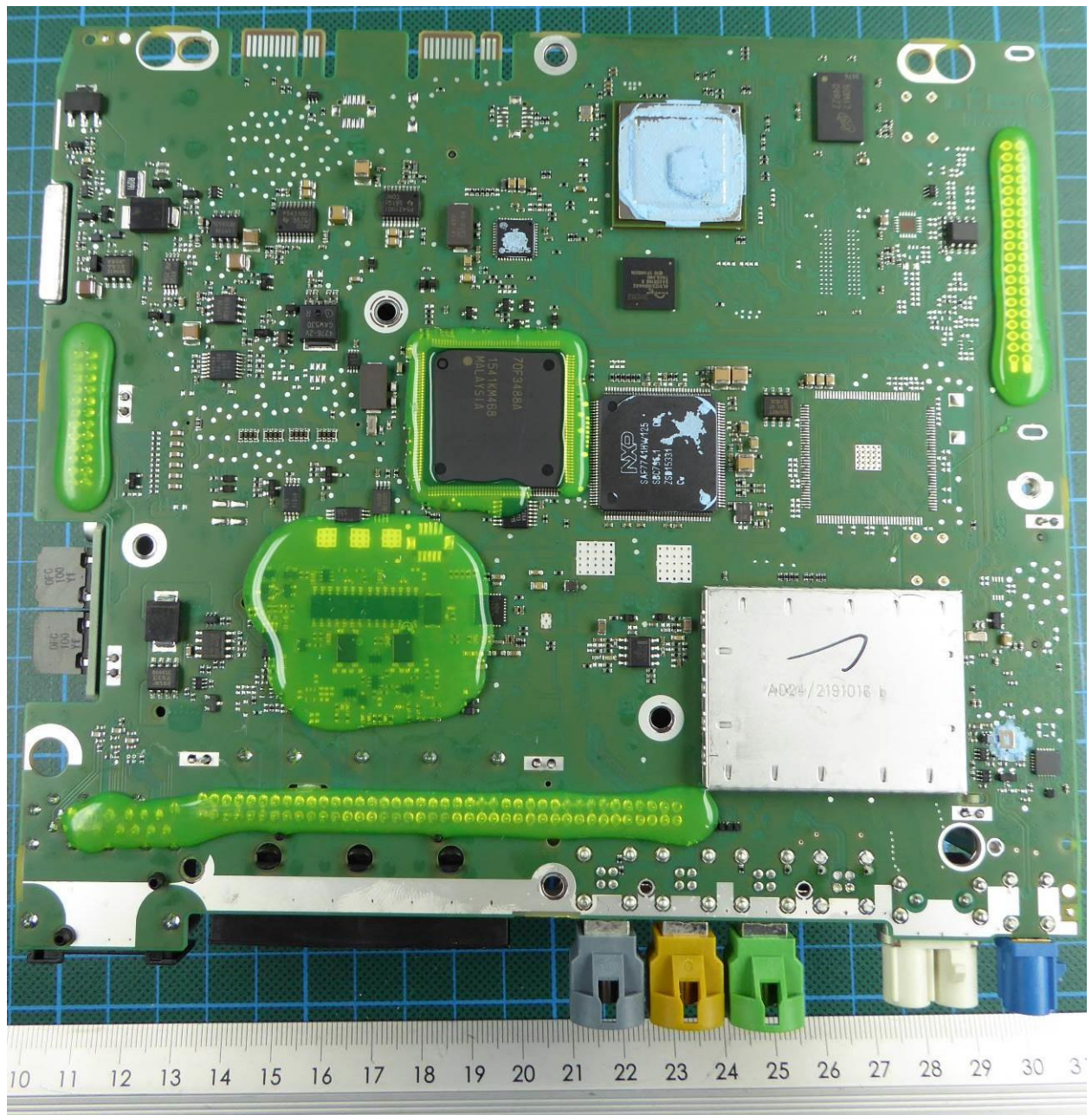
160090_39. jpg: EUT – Main Unit – Main PCB bottom view
