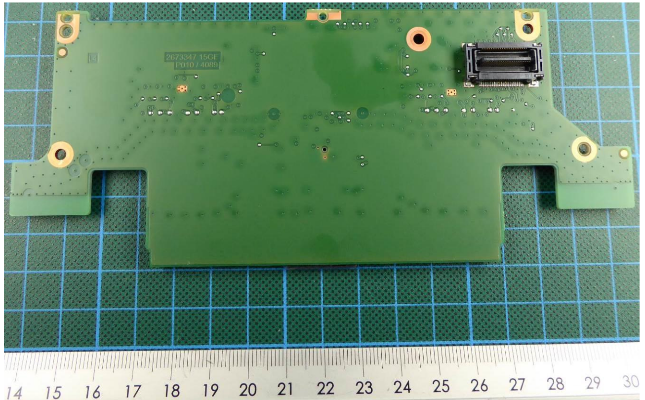
160090_33. jpg: EUT – Main Unit – RF PCB bottom view
