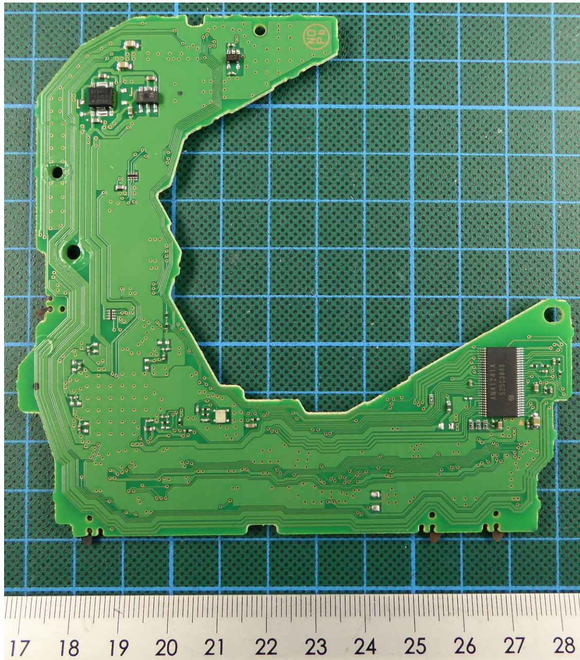
160090_27. jpg: EUT – Main Unit – CD drive PCB bottom view
