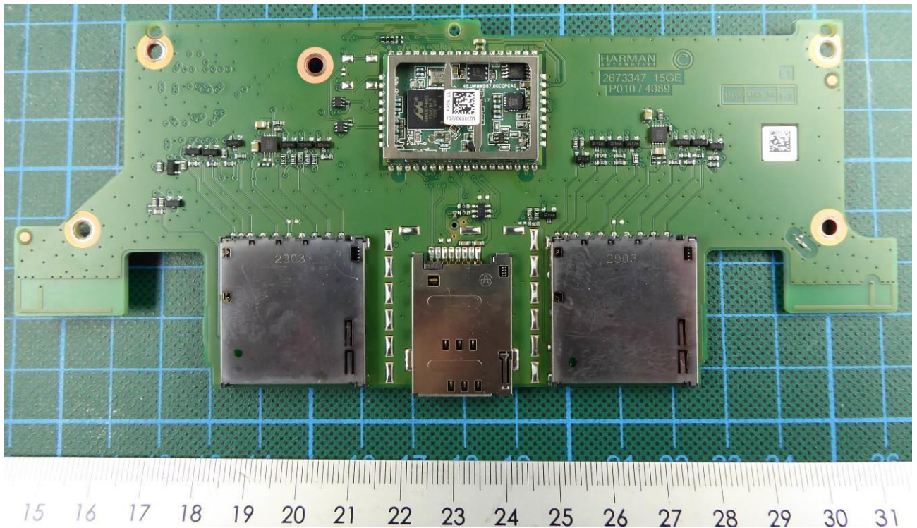
160090_34. jpg: EUT – Main Unit – RF PCB top view without shielding
