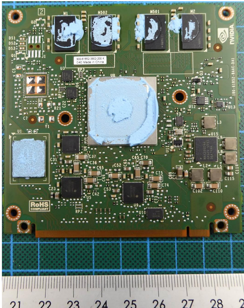
160090_36. jpg: EUT – Main Unit – Computing PCB top view
