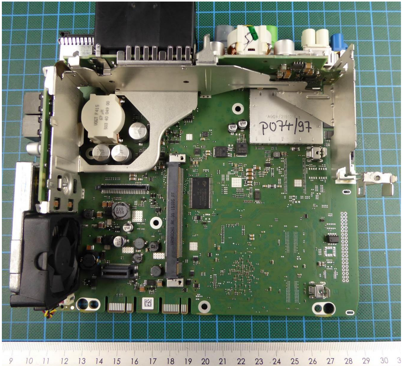
160090_38. jpg: EUT – Main Unit – Main PCB top view
