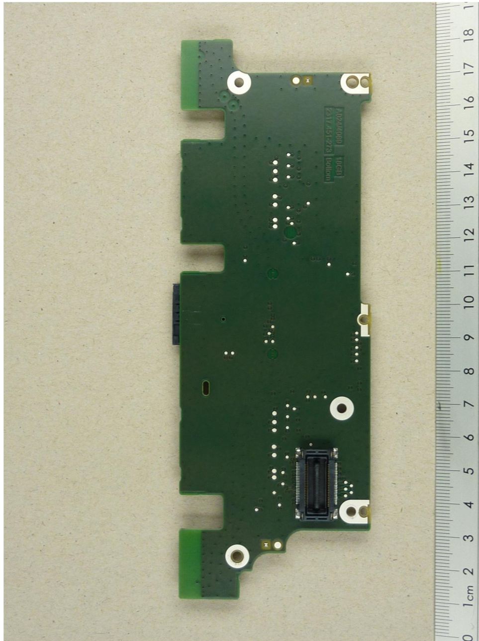
123736_10.JPG: Audi MIB, WLAN/BT board, bottom view
