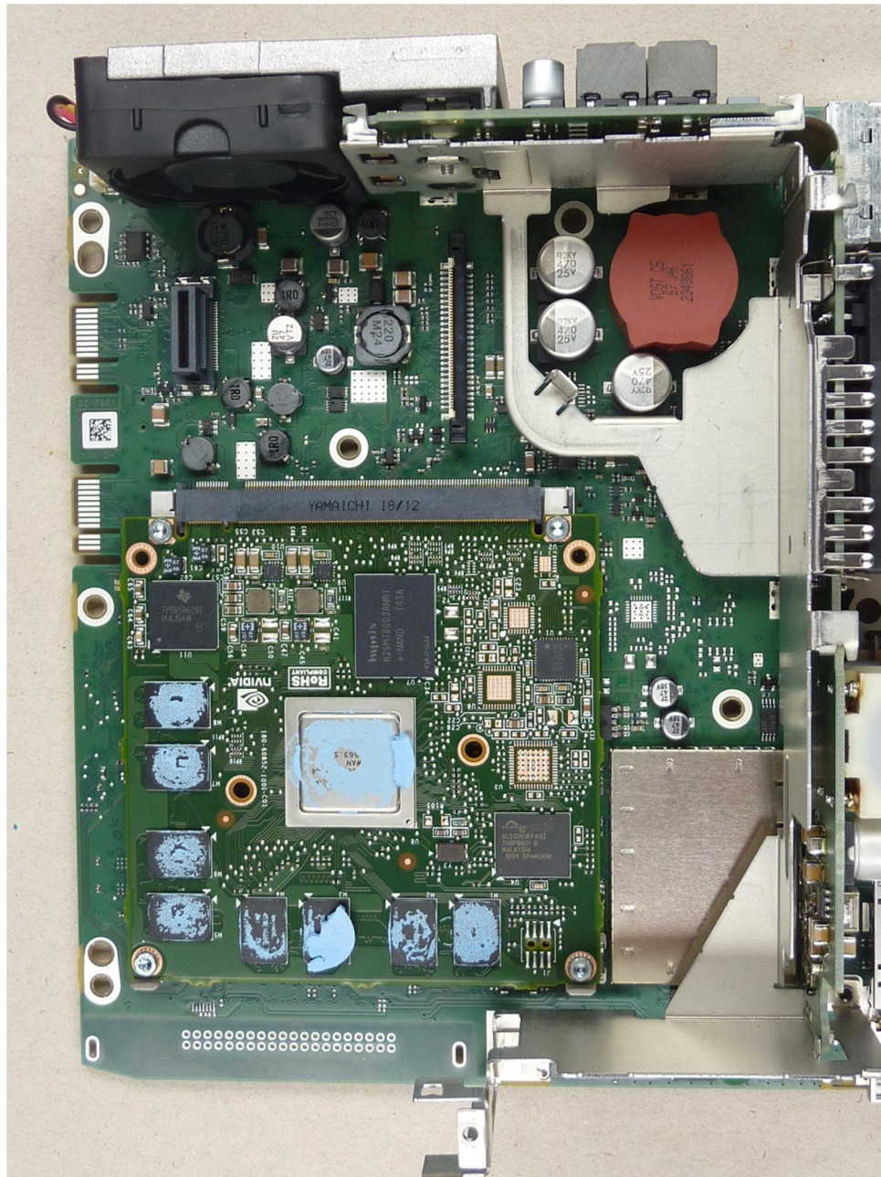
123736_35.JPG: Audi MIB, main PCB, top view
