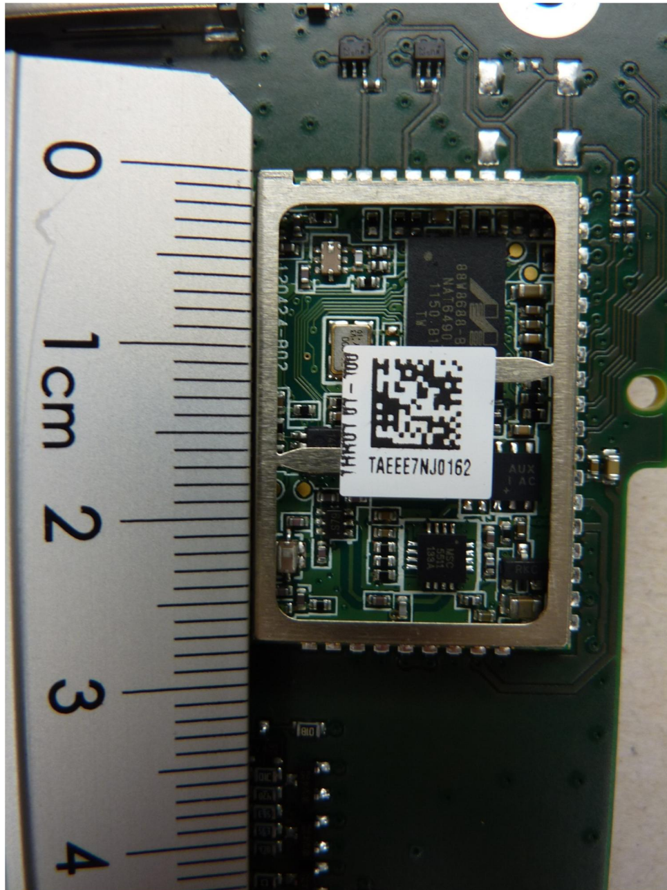
123736_9.JPG: Audi MIB, detail view to WLAN/BT circuit
