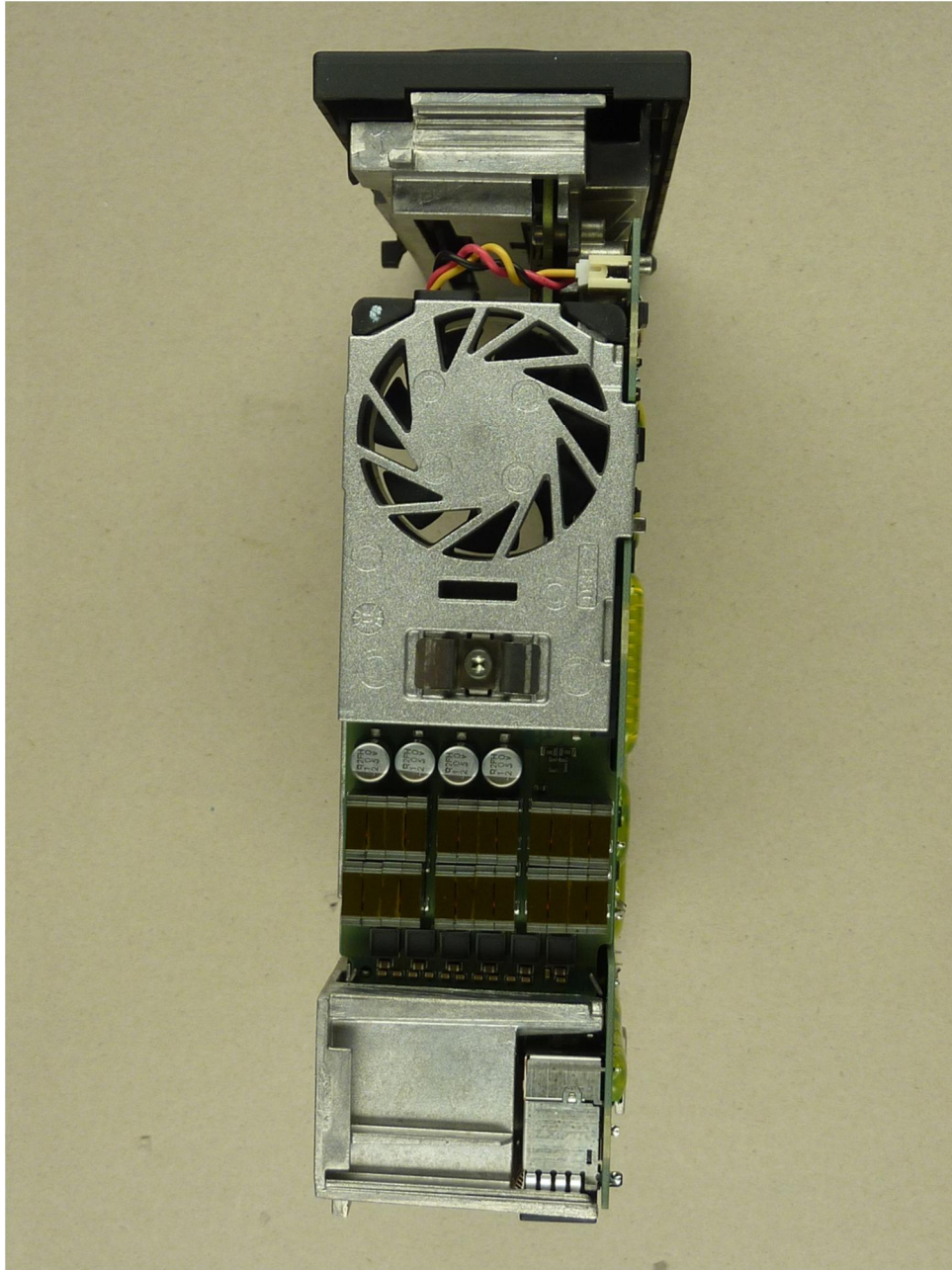
123736_32.JPG: Audi MIB, left hand view with removed top cover
