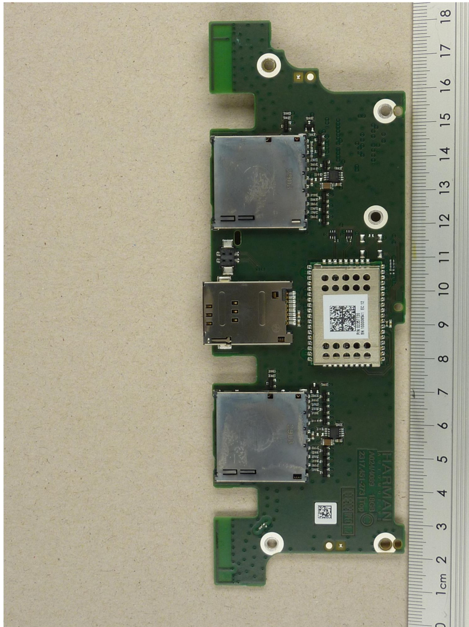
123736_8.JPG: Audi MIB, WLAN/BT board, top view
