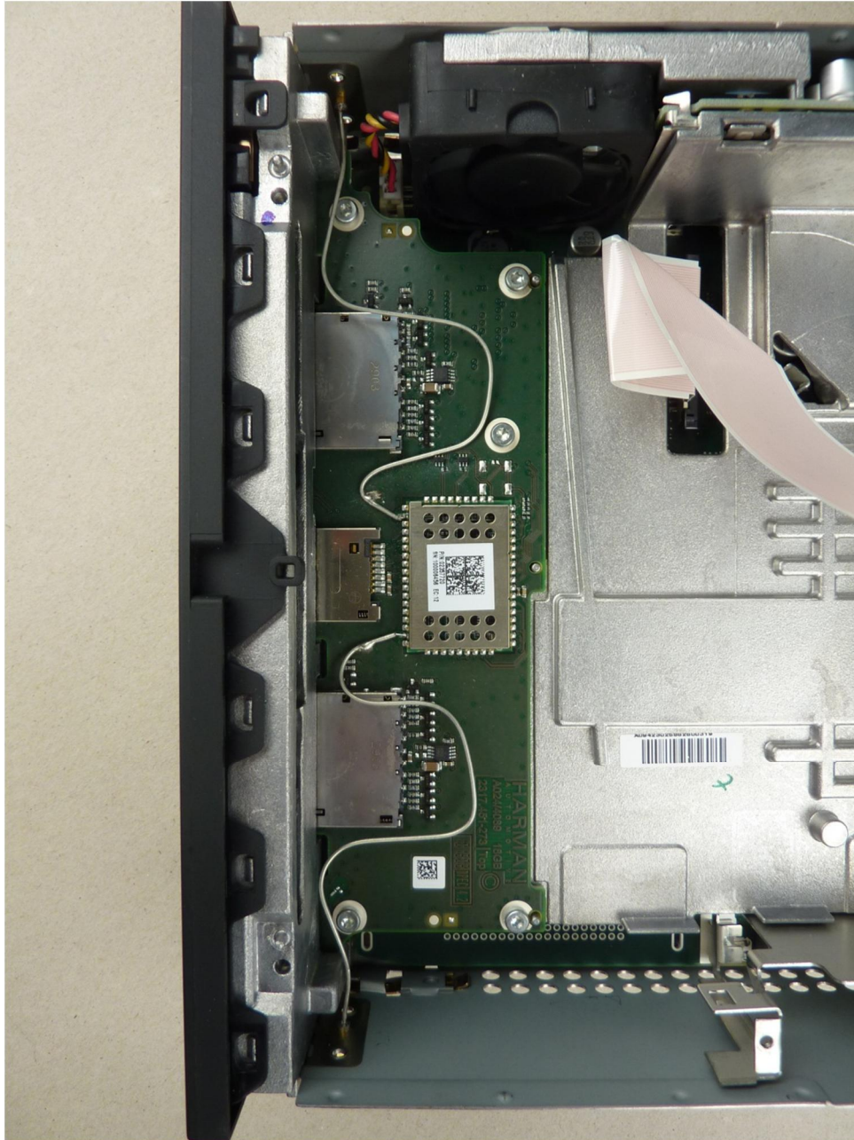
123736_16.JPG: Audi MIB, detail view to temporary antenna connectors
