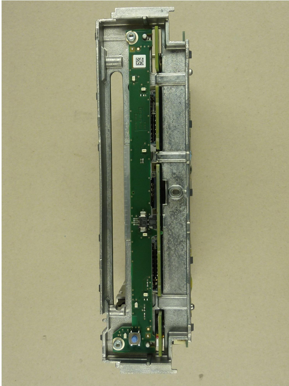
123736_33.JPG: Audi MIB, front cover removed
