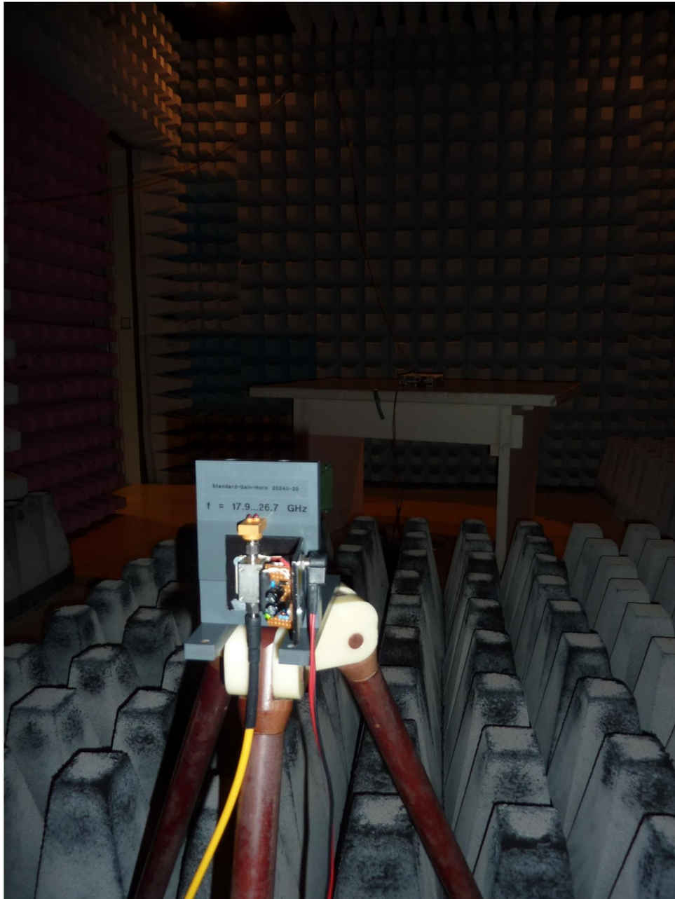
123736_5.JPG: Test setup fully anechoic chamber
