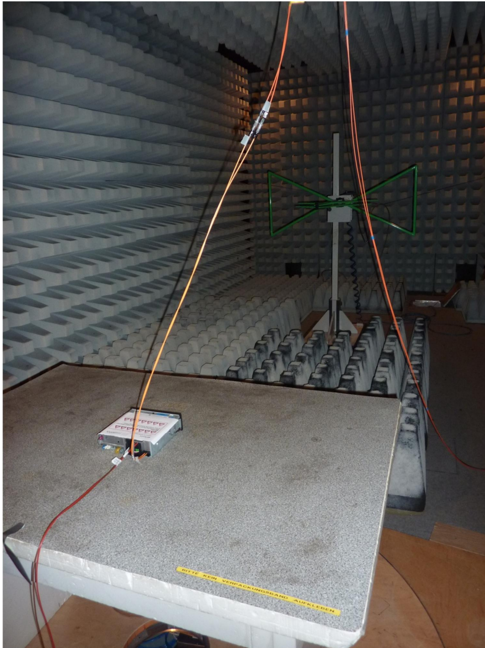
123736_2.JPG: Test setup fully anechoic chamber
