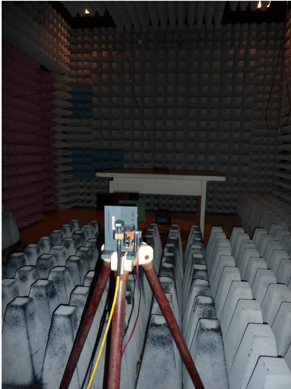
123736_4.JPG: Test setup fully anechoic chamber
