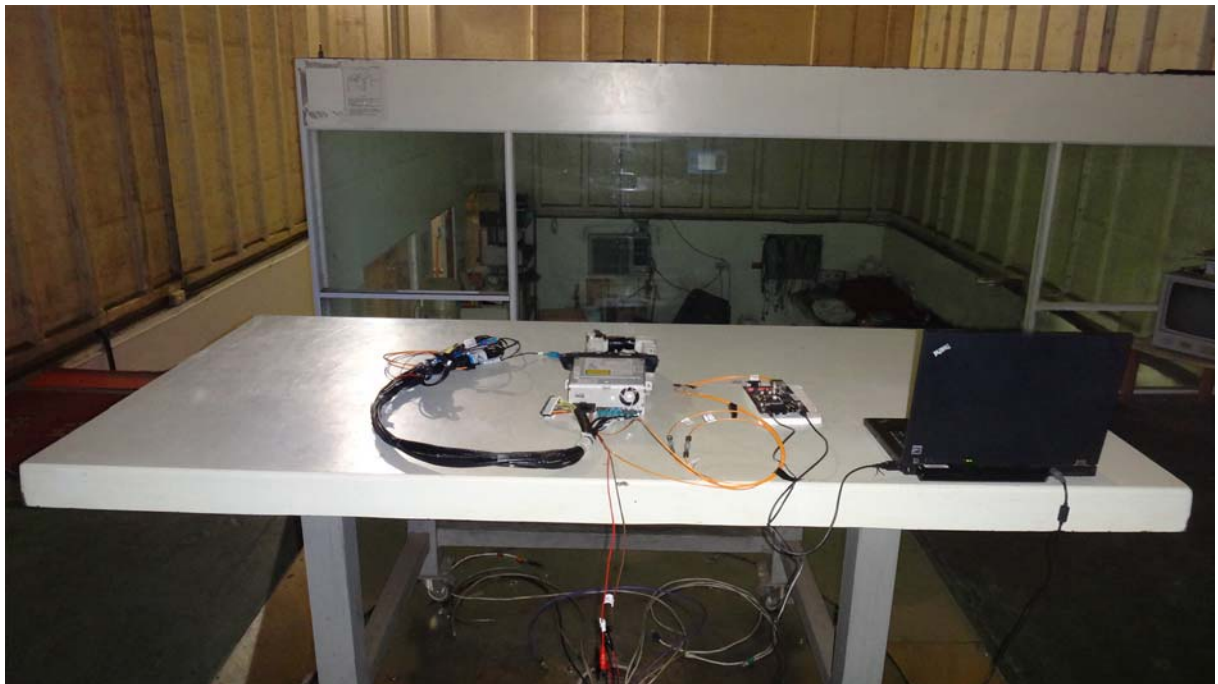
Back View of Radiated Test
