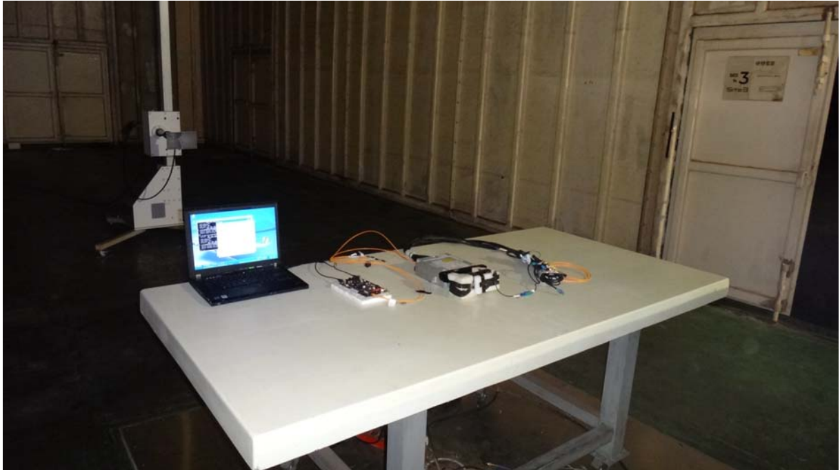
" Front View of Radiated Test (Horn)"
