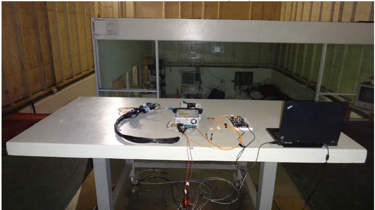
" Back View of Radiated Test (Horn)"
