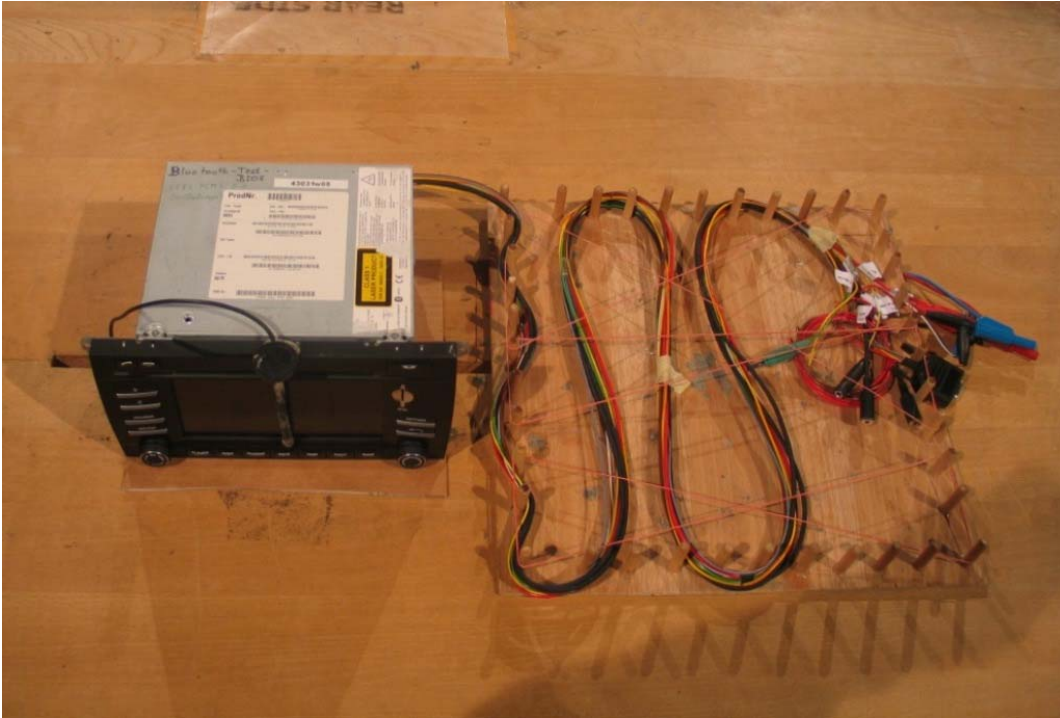
Photo 1: Test setup for radiated measurements (Enclosure, 30 MHz to 1 GHz)
