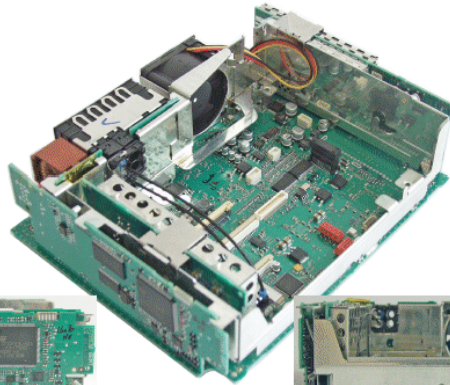
IO-Controllerboard 4110-bs
