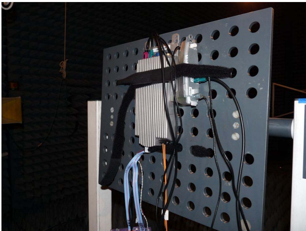
PHOTO No. 1: Set-up for radiated tests
