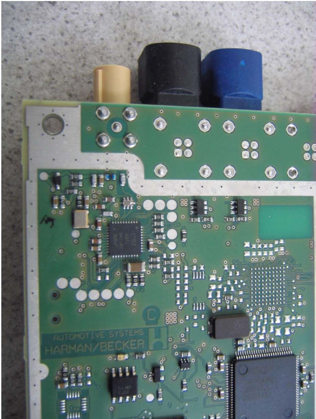
Details of BT-Part
