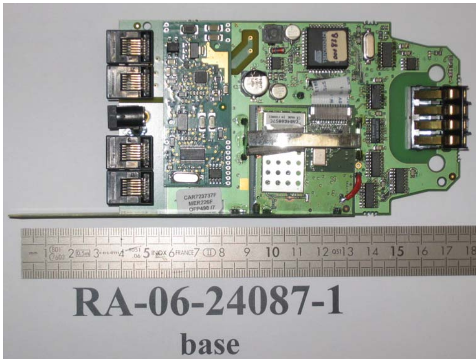
Printed circuit of the base
