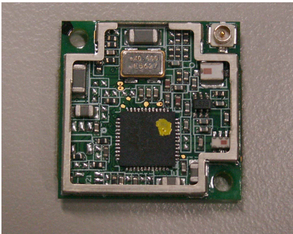
RF Part without Shield (Top)
