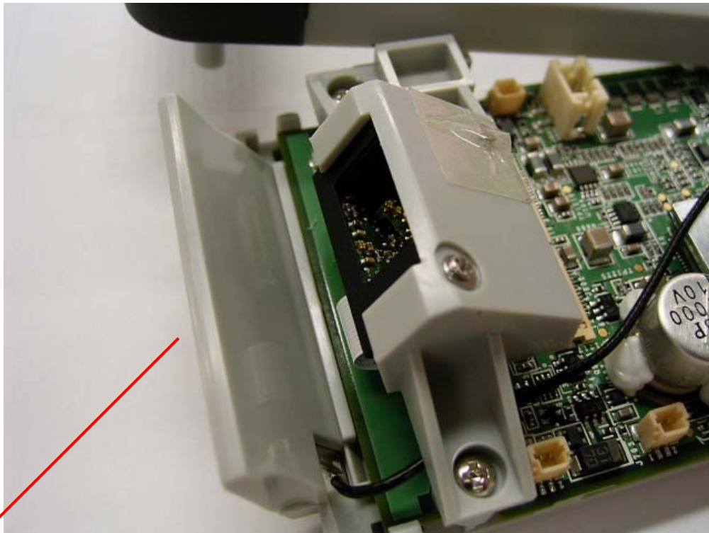
Antenna Location (Top)
