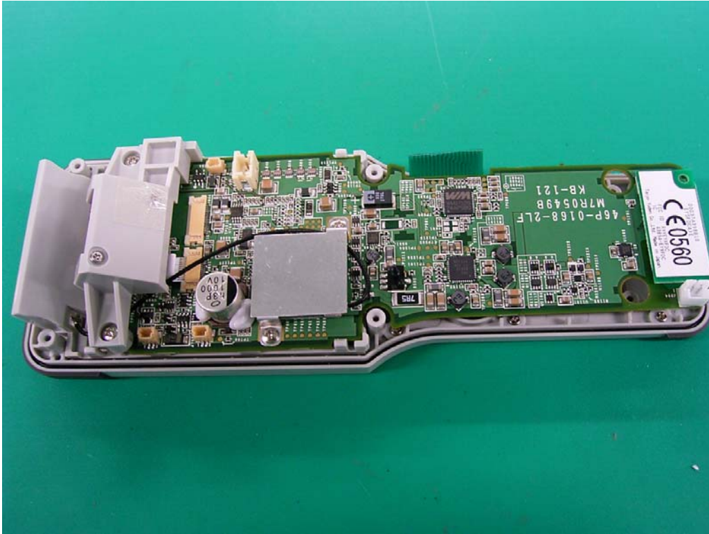
Overall (Top)
