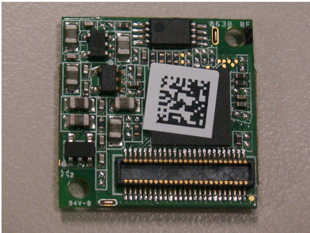
RF Part (Bottom)
