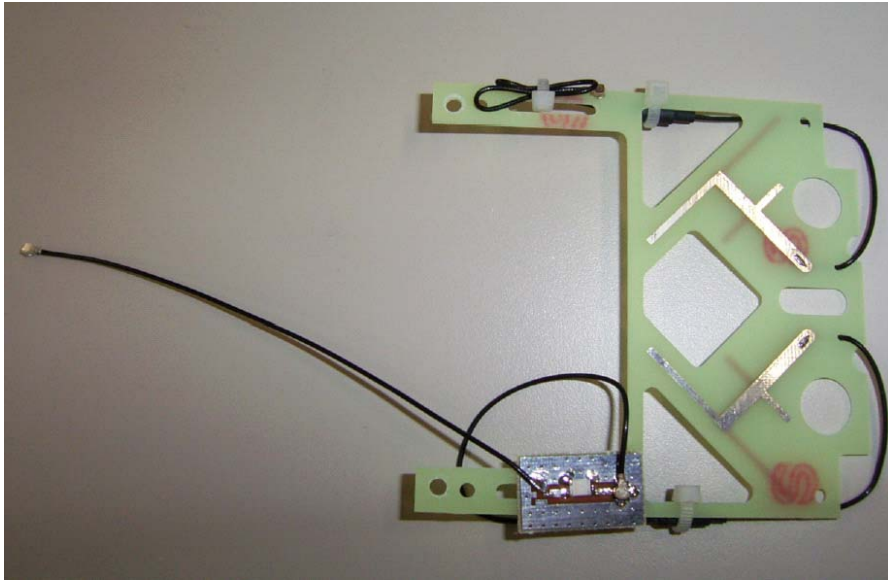
Antenna (Front)
