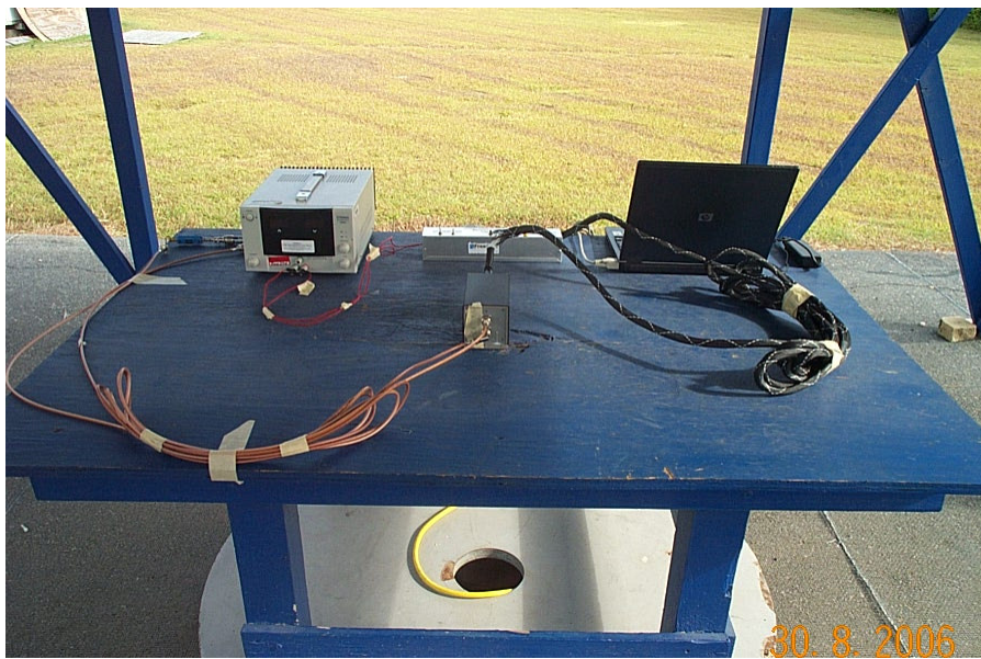
Radiated Measurement Setup – Back
