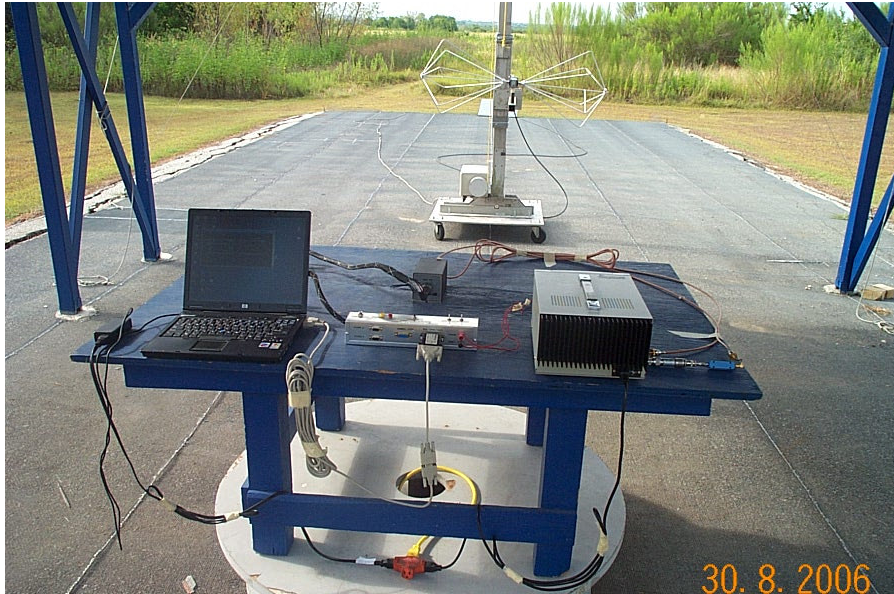
Radiated Measurement Setup - Front
