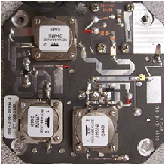
Fig 8 – 1900-3108-00
