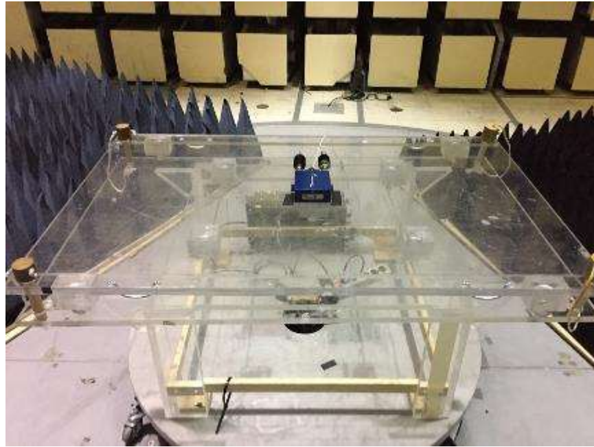
Radiated Measurements up to 1 GHz, Front
