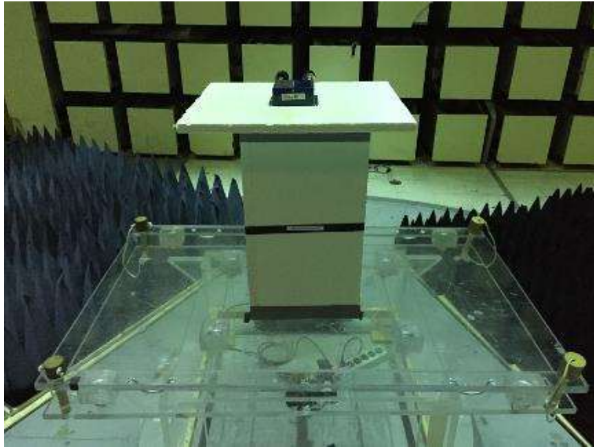
Radiated Measurements, Above 1 GHz, Front
