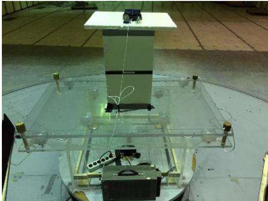
Radiated Measurements, Above 1 GHz, Back
