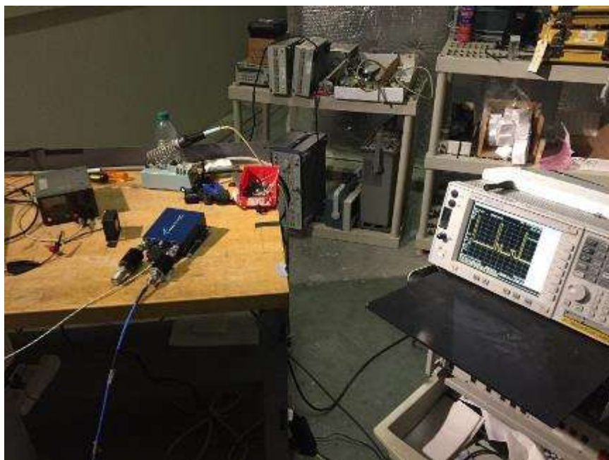
Conducted Antenna Port Measurements, Power, BW, Spurious, Mask Top Port (right)
