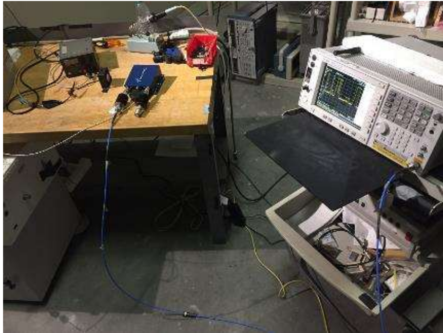
Conducted Antenna Port Measurements, Power, BW, Spurious, Mask Bottom Port (left)
