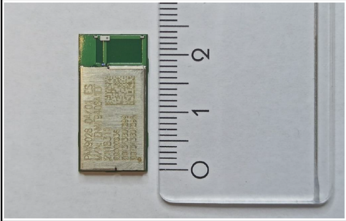
ENWF9408A1EF_top_case
