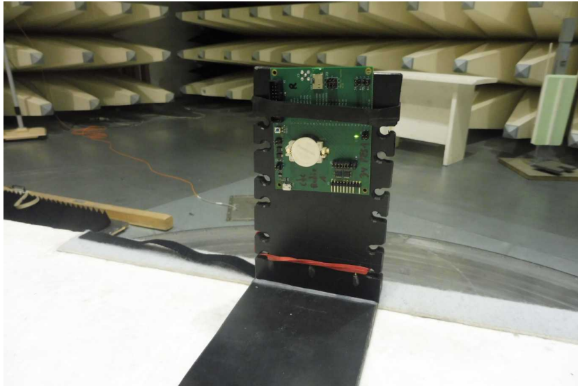
Photo 7 RSE < 1GHz
