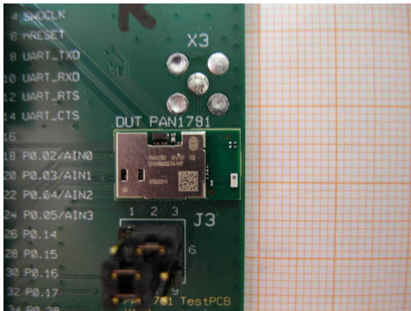
Photo 2 radiated Sample
