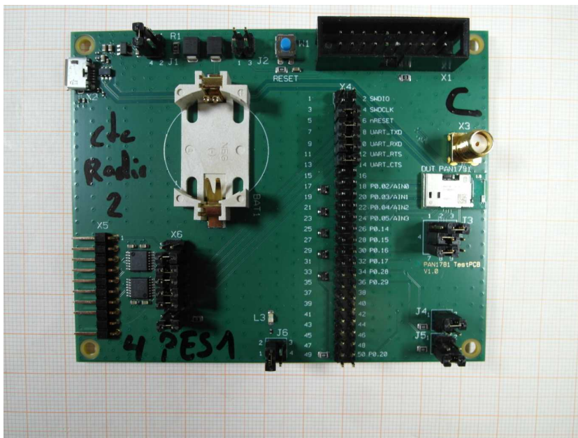
Photo 4 conducted Sample
