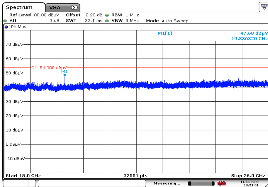
Plot 12: 18 GHz to 26 GHz, TX mode, 2480 MHz, vertical & horizontal polarization, 2 Msp
