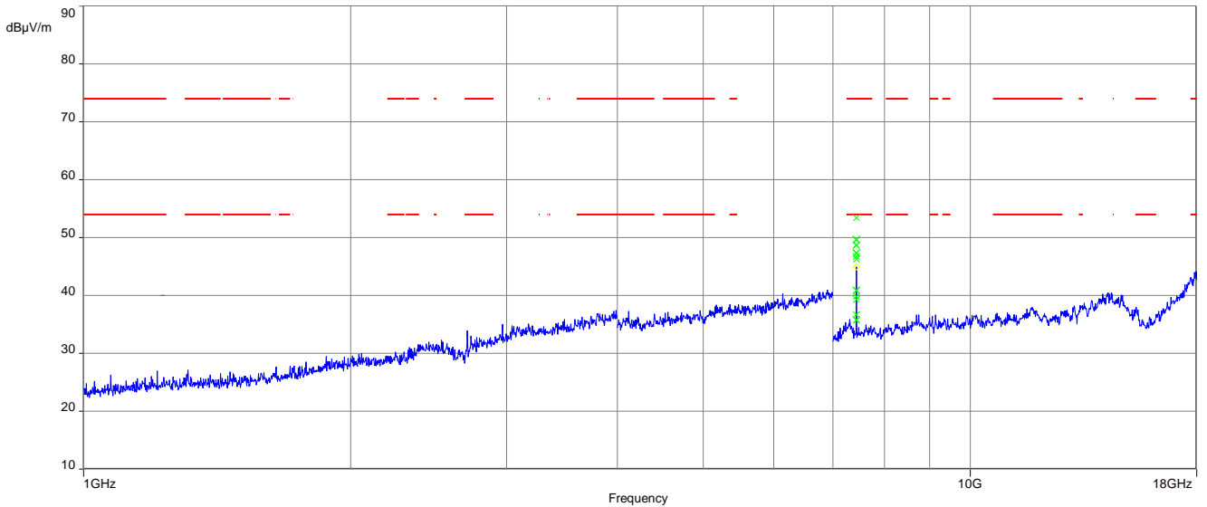
Plot 11: 1 GHz to 18 GHz, TX mode, 2480 MHz, vertical & horizontal polarization, 2 Msp
