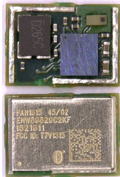
EUT PAN 1315 - ENW89829C2KF with and without shielding
