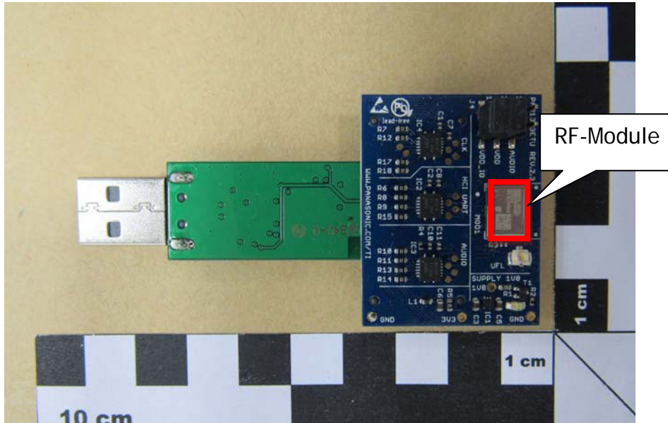
PAN 1315 - ENW89829C3KF ON EVALUATION BOARD TOP
