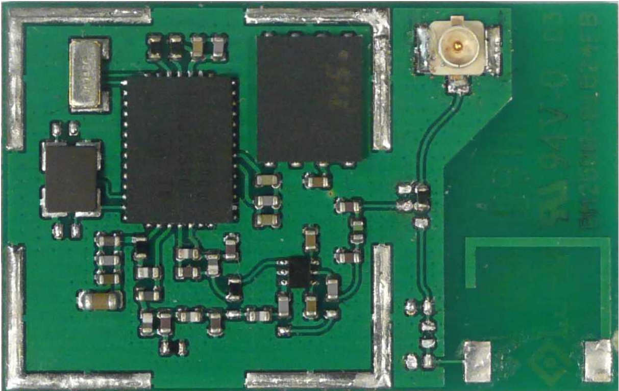
PAN2580 with UFL-connector (ENW59625BxDF)
