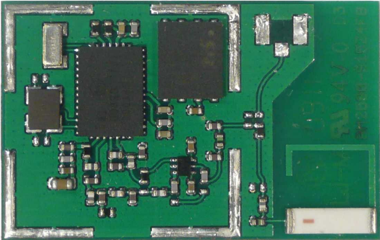
PAN2580 with ceramic-antenna (ENW59625AxDF)
