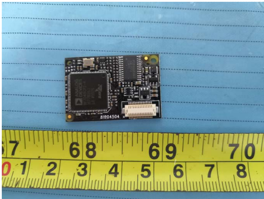
EUT – DSP Board Top View
