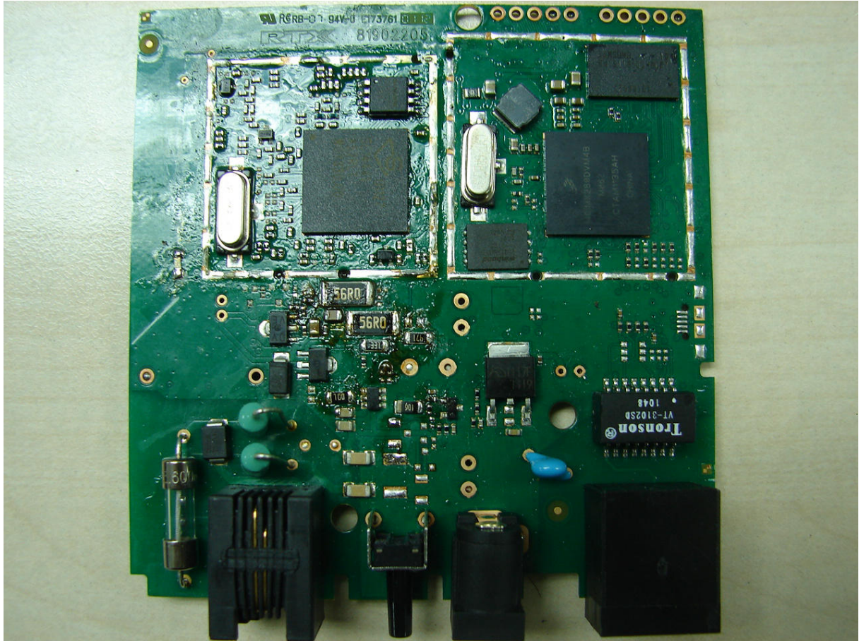
Internal view without shielding
