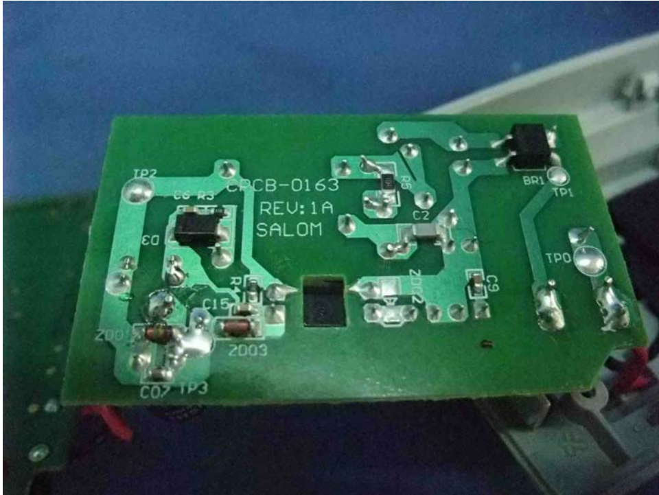
Telephone Line Extender an other Main PCB solder side
