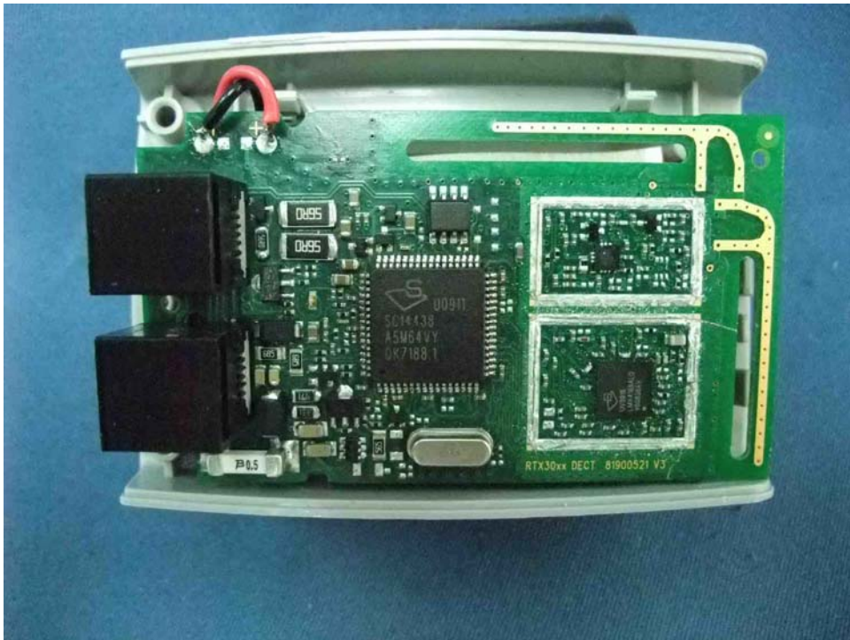
Telephone Line Extender Main PCB comp side
