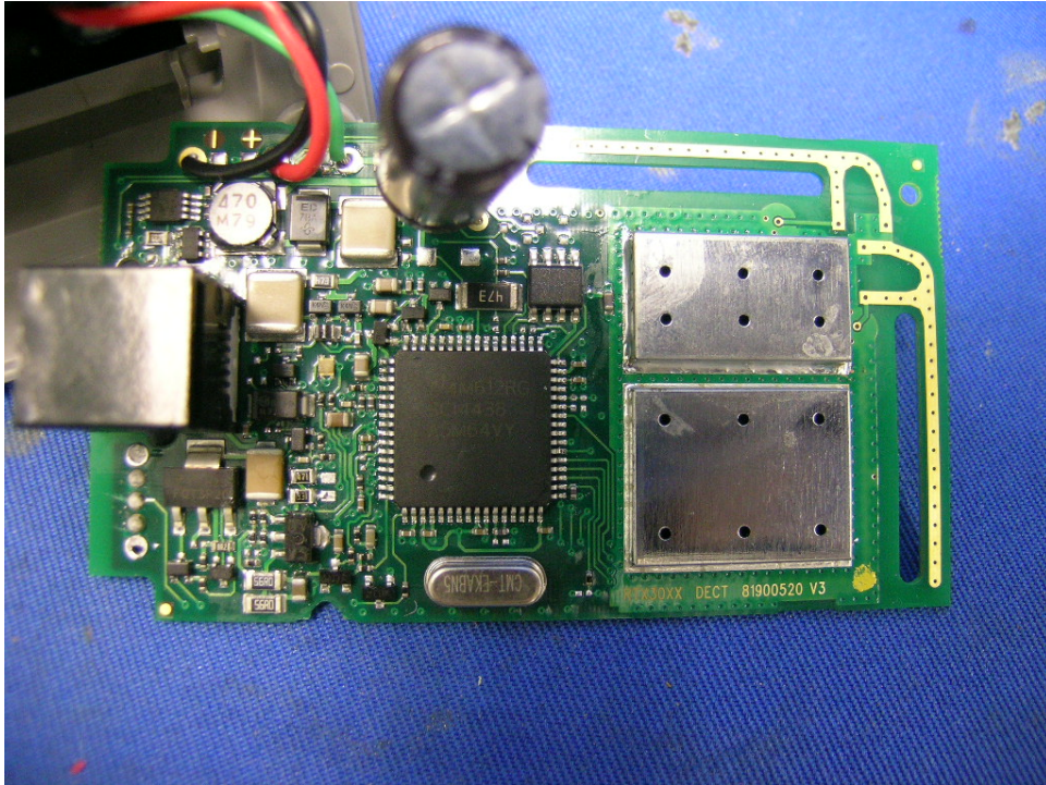
Extension Unit Main PCB comp side (View 2)
