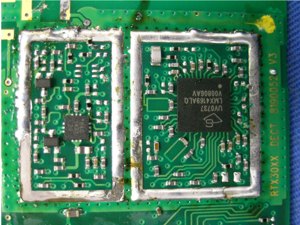
Extension Unit Oscillator PCB comp side
