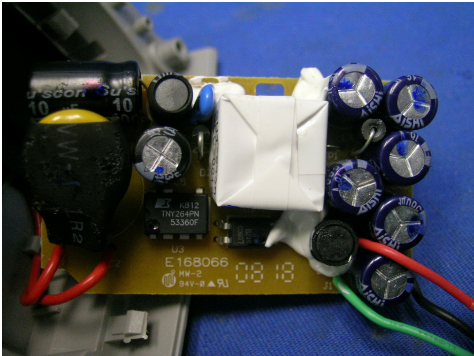
Extension Unit Power Board front side
