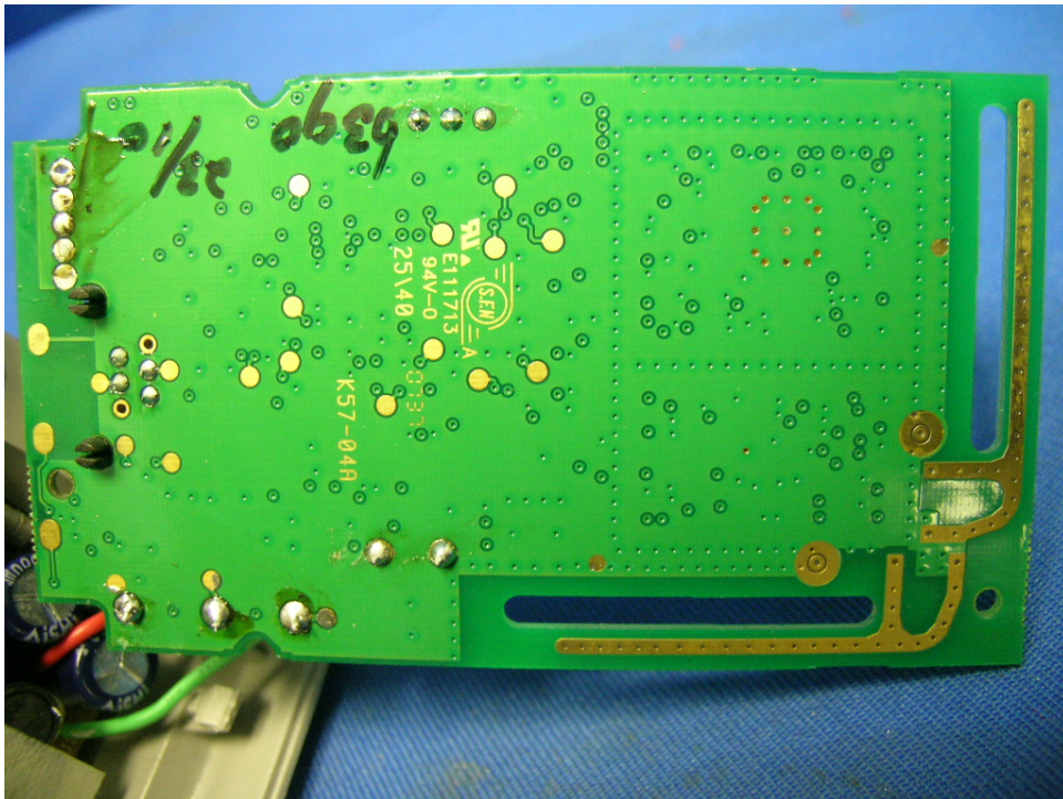
Extension Unit Main PCB solder side
