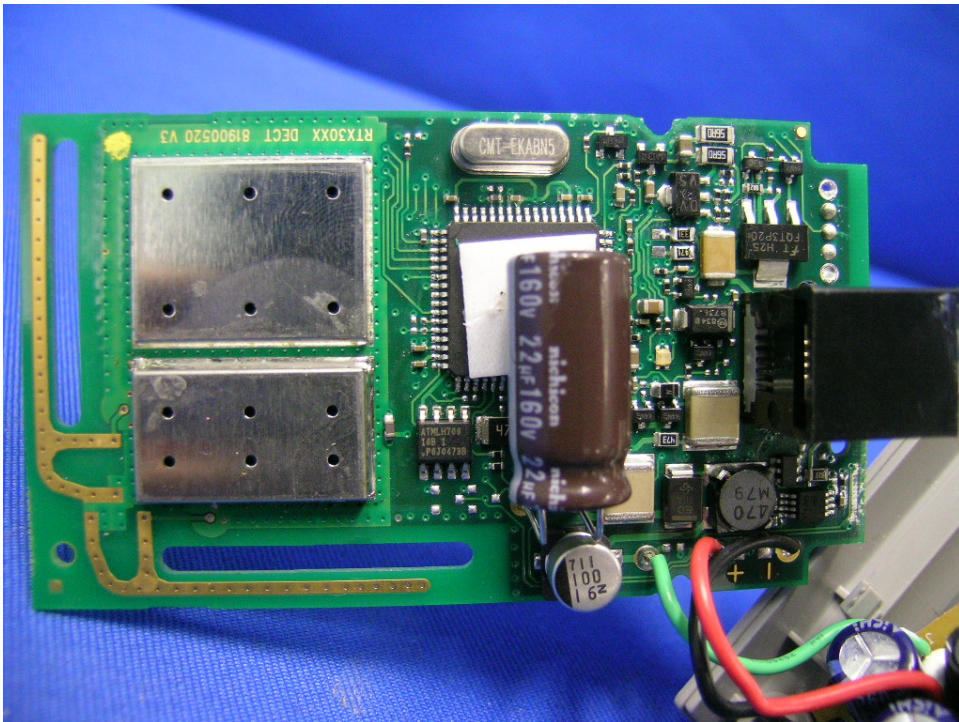
Extension Unit Main PCB comp side (View 1)
