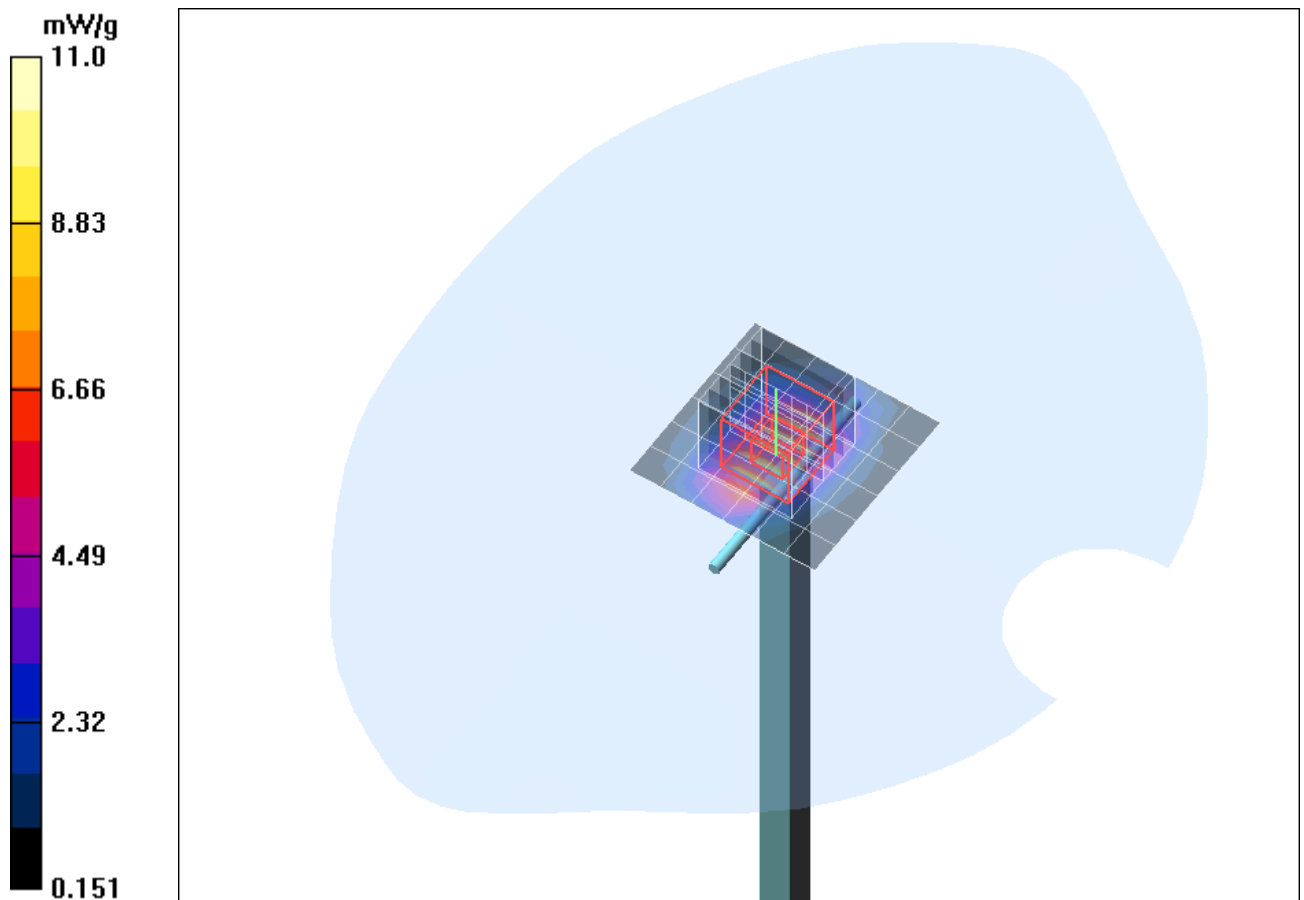
Fig. 10: Validation measurement 1900 MHz Head (March 29, 2011), coarse grid.
