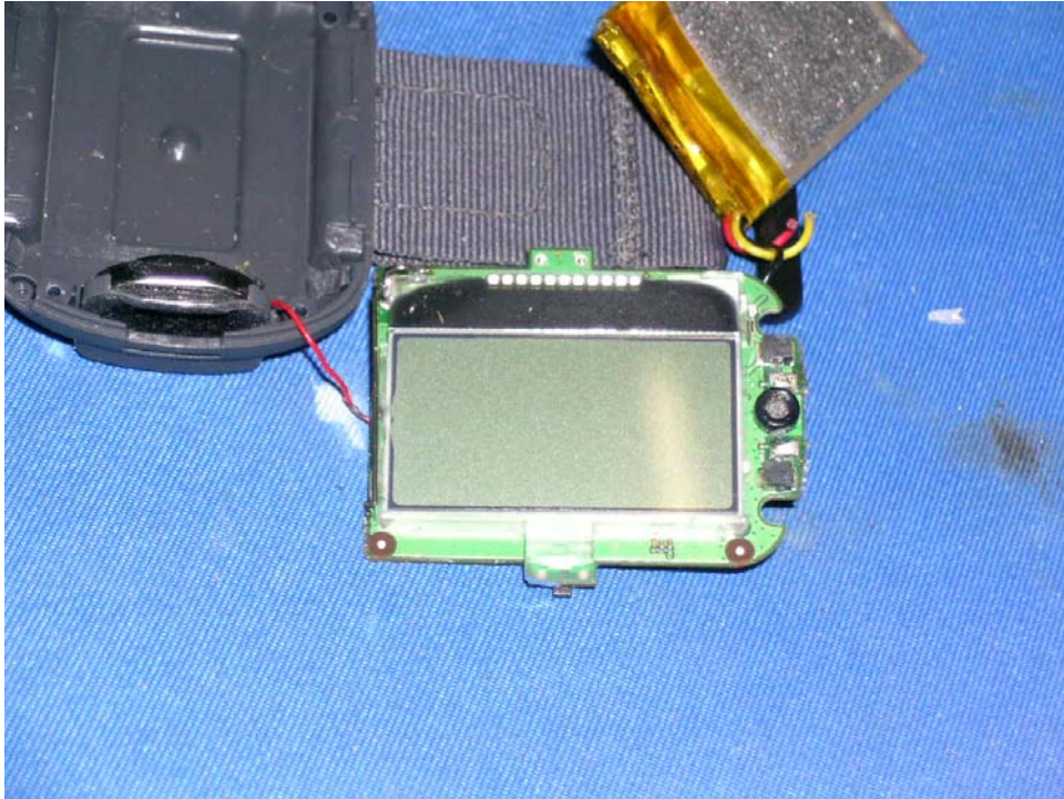
DECT Messenger LCD Display comp side (View 1)
