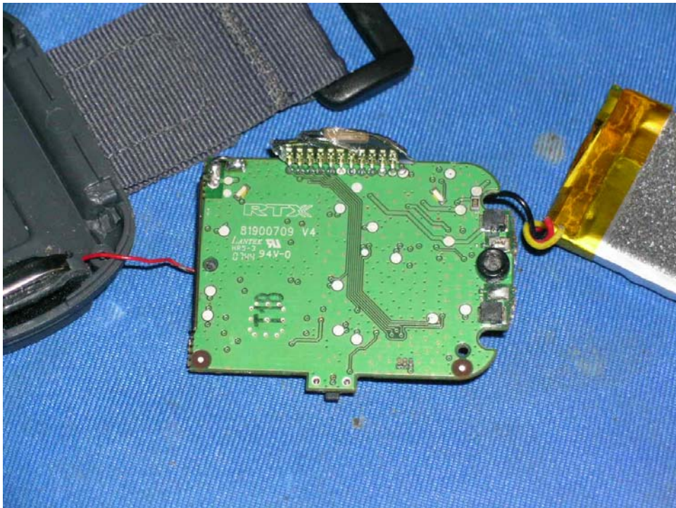
DECT Messenger LCD Display comp side (View 2)
