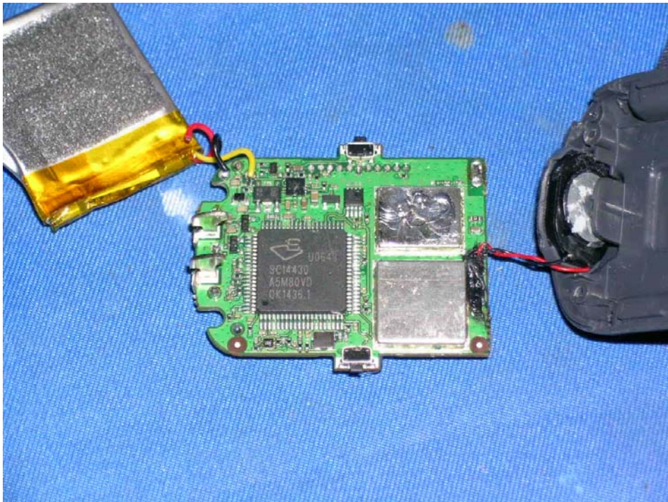
DECT Messenger Main PCB comp side
