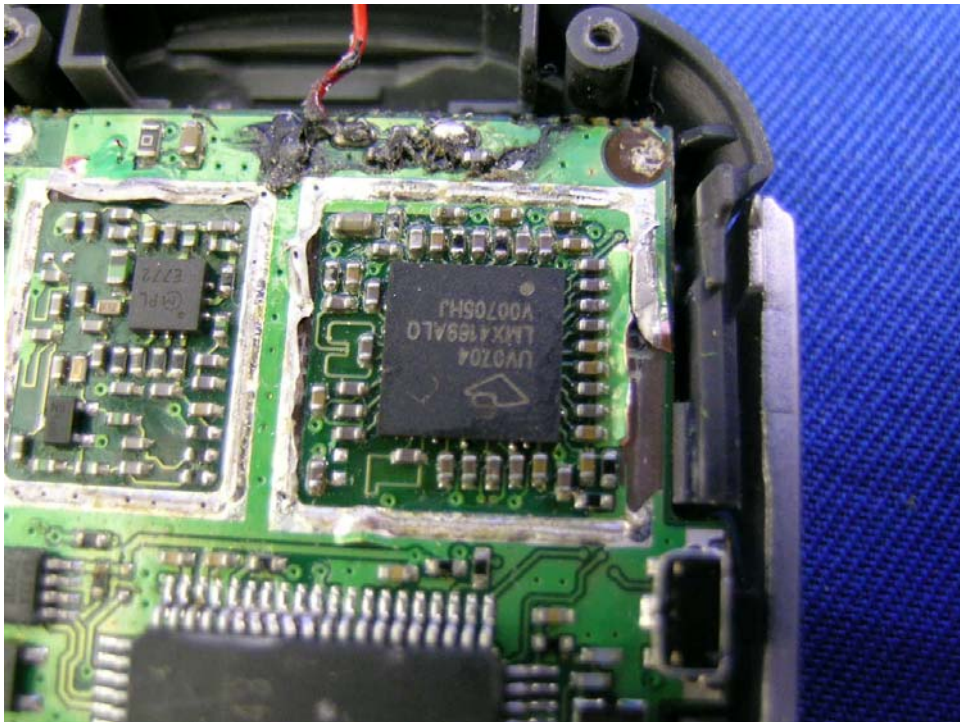
DECT Messenger Oscillator PCB comp side (View 2)
