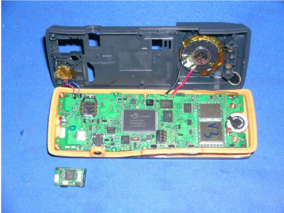
Handset assembly (View 3)
