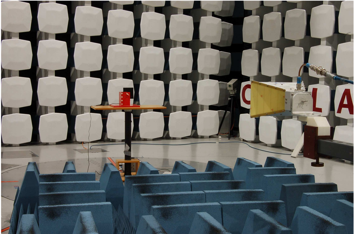
Antenna Gain Test
