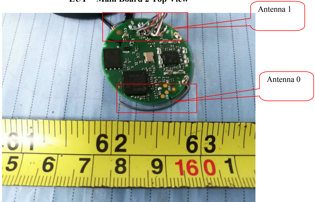
EUT – Main Board 2 Top View
