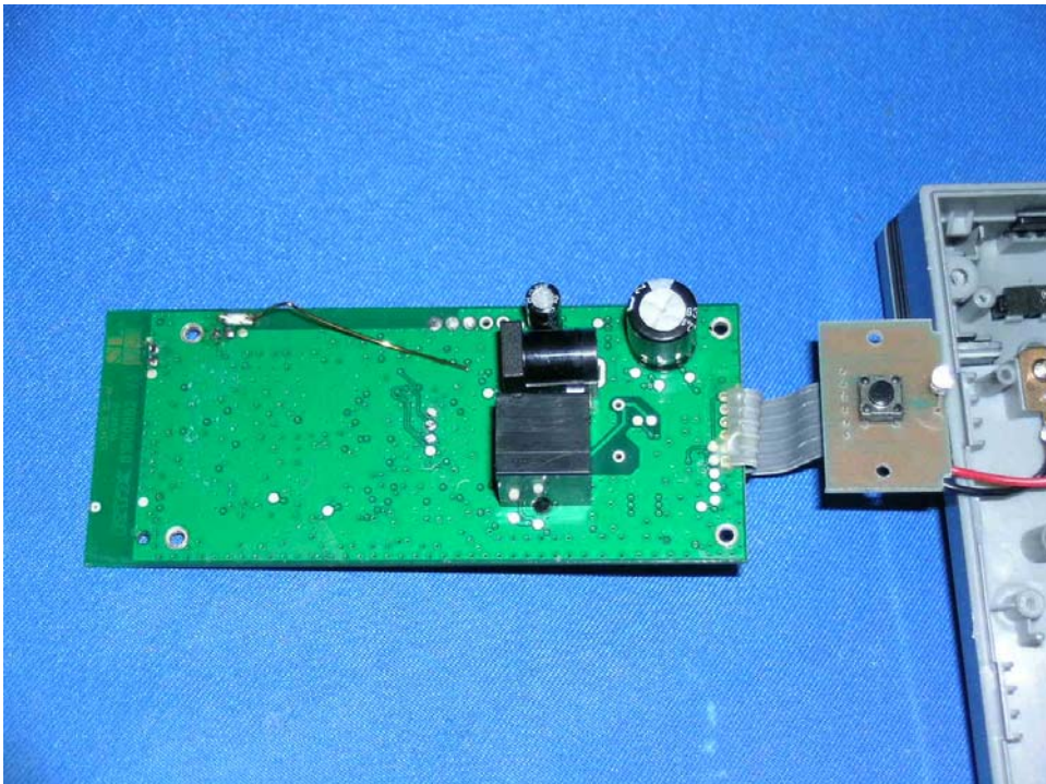
Base Unit Main PCB and Page Key comp side
